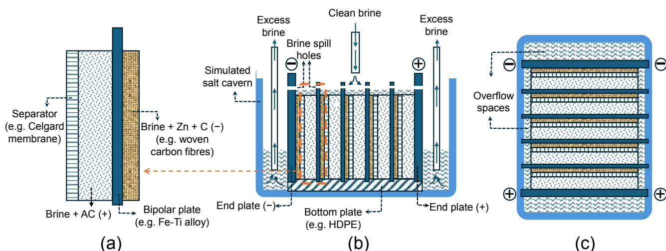
Figure 9. Laboratory simulated salt cavern supercapattery stack with bipolarly connected 5 Zn | AC cells. (a) Cross section view of the repeating bipolar plate (electrode) assembly in the bipolar stack. (b) Cross section and (c) top views of the bipolar stack. (HDPE: High density polyethylene.)
