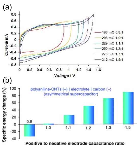
Figure 8. (a) CVs and (b) the specific energy of the cell of “polyaniline/carbon nanotubes | 1.0 M HCl | carbon” at the indicated positrode to negatrode capacitance ratios. Reproduced from ref. 137 with permission from RSC Publishing, copyright 2010.
