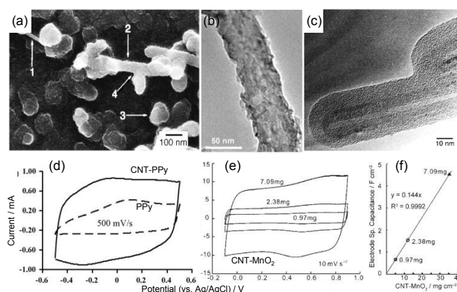
Figure 4. TEM images of carbon nanotubes (CNTs) coated with (a) polypyrrole (CNT-PPy), reproduced from ref. 71 with permission from John Wiley and Sons, copyright 2000, and (b) manganese dioxide (CNT-MnO 2 ), reproduced from ref. 70 with permission from John Wiley and Sons, copyright 2007. The HRTEM image in (c) 71 confirms the enclosure of individual CNTs by uniform PPy coatings. Cyclic voltammograms were obtained from (d) pure PPy and CNT-PPy of same deposition charge in aqueous 0.5 \text{ mol L}^{-1} \text{ KCl} , 88 and (e) CNT-MnO 2 in aqueous 2.0 \text{ mol L}^{-1} \text{ KCl} at different overall loadings which are translated to the respective areal loadings in (f). 70 Reproduced from ref. 71 with permission from John Wiley and Sons, copyright 2000, from ref. 88 with permission from Elsevier,
