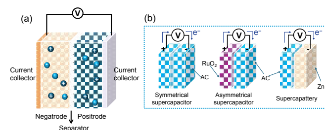
Figure 2. Schematic illustrations of (a) the structure of a generic EES device (cell) and (b) charging three different EES devices as indicated.
