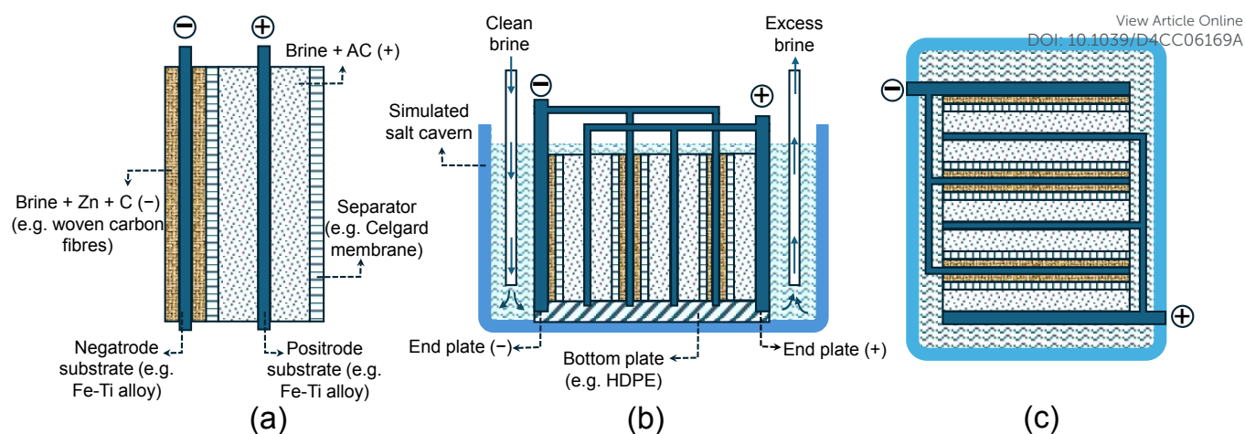
Figure 10. Laboratory simulated salt cavern supercapattery stack with 5 Zn||AC cells in parallel connection. (a) Cross section view of the repeating parallel plates (electrodes) assembly. (b) Cross section and (c) top views of the parallel stack. HDPE: High density polyethylene
