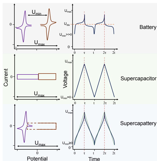
Figure 3. Illustration of CVs of electrodes and GCD profiles of two-electrode cells of battery, supercapacitor and supercapattery. (Redrawn from Ref. 50 )
