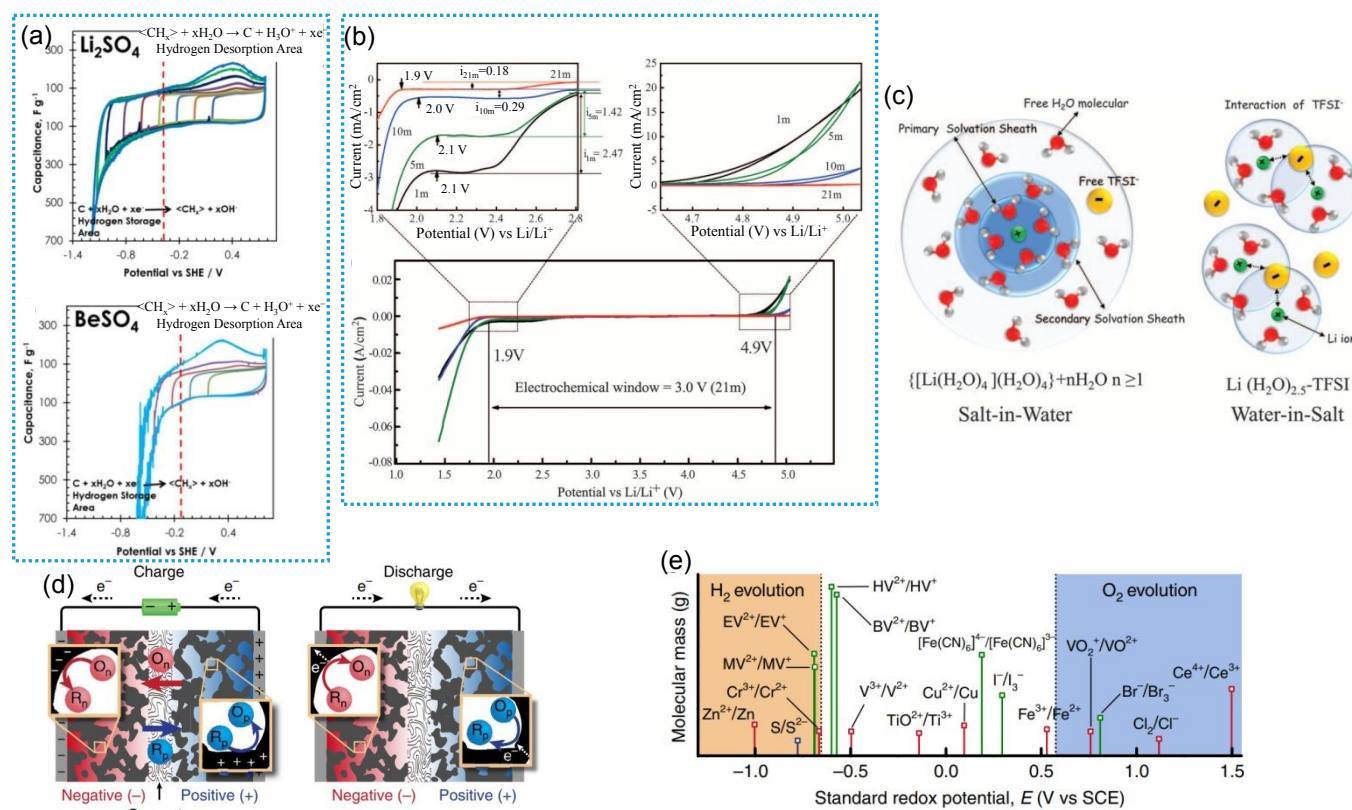
Figure 7. (a) CVs of AC at 2 mV s -1 in 1 M \text{Li}_2\text{SO}_4 with pH = 6.5 (left) and in 1 M \text{BeSO}_4 with pH = 2.1 (right). Reproduced from ref. 106 with permission from IOP Publishing, copyright 2015. (b) The HER and OER potentials and electrochemical window of WIS electrolytes. (c) Illustration of the Li + solvation sheath in diluted and water-in-salt solutions. Reproduced from ref. 108 with permission from Springer Nature, copyright 2013. (d) Schematic of the capacitive and faradaic charge storage processes with redox couple in the electrolyte. (e) Reduction potentials of the indicated redox couples. (BV, benzyl viologen; EV, ethyl viologen; HV, heptyl viologen; MV, methyl viologen) Reproduced from ref. 114 with permission from Springer Nature, copyright 2015.
