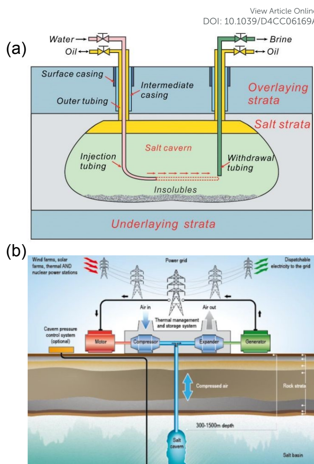
Figure 1. Schematic illustrations of (a) two well horizontal salt cavern construction, reproduced from ref. 25 with permission from Taylor & Francis, copyright 2020 and (b) compressed air energy storage in salt caverns, reproduced from ref. 26 with permission from Elsevier, copyright 2021.
