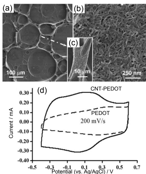
Figure 5. SEM images of electro-deposited CNT-PEDOT films from a CNTs assisted metastable emulsion, showing (a) interconnected craters of various sizes with enlarged views of (b) the base and the bank of the crater. Reproduced from ref. 91 with permission
