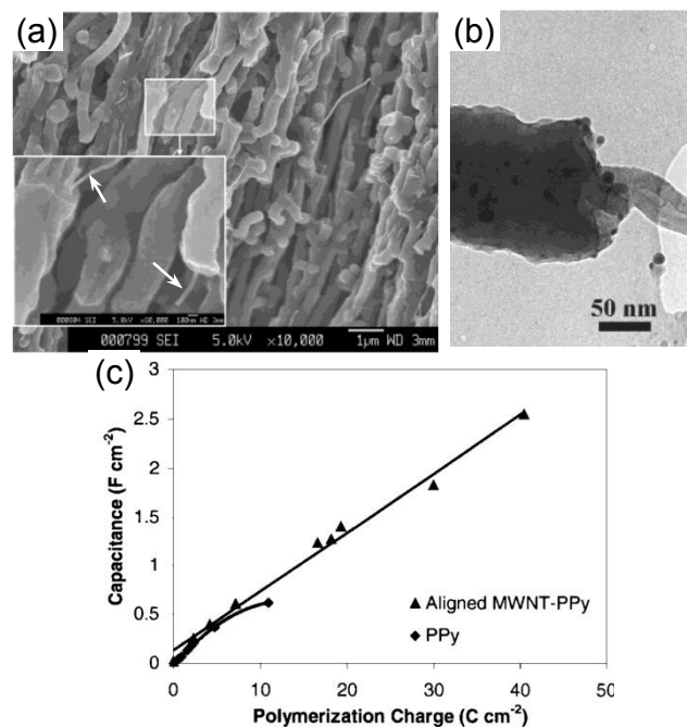
Figure 6. (a) SEM images of vertically aligned CNTs coated with PPy via direct electro-deposition (deposition charge: 40 \text{ C cm}^{-2} ). The inset is an enlarged view showing the uncoated portions of the CNTs. (b) A single CNT with the left portion being coated with PPy and the right portion being naked. (c) Areal capacitance of PPy coated vertically aligned CNTs (triangles) and that of pure PPy (diamonds) as a function of deposition charge. Reproduced from ref. 92 with permission from John Wiley and Sons, copyright 2002.
