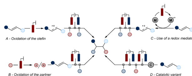
Fig. 1 General representation of the possible oxidative electrochemical pathways for the functionalization of olefins.
