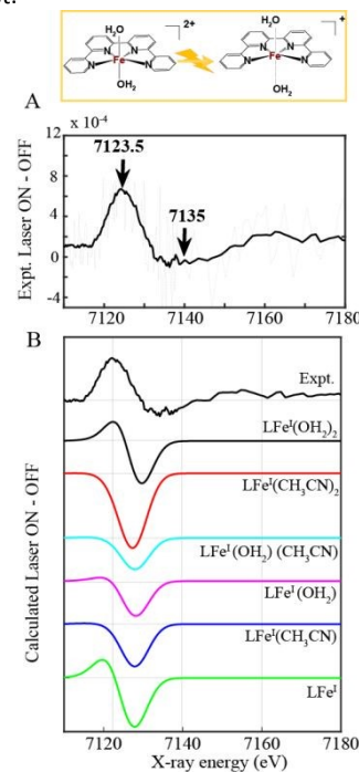
Fig. 4. Top. Formation of a photoreduced \text{Fe}^{\text{I}} species with 2 loosely coordinated molecules for a multimolecular assembly composed of 2.5 mM AI-1 photosensitizer, 1 mM FeQPY catalyst, 100 mM BIH and 100 mM TEOA in a solution mixture of 0.93:0.07 \text{CH}_3\text{CN} :DMF. A small amount of DMF is added to help improve the solubility of the AI -based photosensitizers used hereby in 2.5 mM concentrations. A similar transient signal was obtained for a complete photocatalytic system with AI-2 as sensitizer. A. Experimental Laser ON-OFF spectra corresponding to formation of \text{Fe}^{\text{I}} at 14.2 \mu\text{s} . B. Experimental Laser ON-OFF spectrum (black) in comparison with theoretical XANES simulations corresponding to the formation of a [\text{LFe}^{\text{I}}(\text{OH}_2)_2] (black), [\text{LFe}^{\text{I}}(\text{CH}_3\text{CN})_2] , [\text{LFe}^{\text{I}}(\text{OH}_2)(\text{CH}_3\text{CN})] (cyan) octahedral complex, a square bipyramidal [\text{LFe}^{\text{I}}\text{-OH}_2] (magenta), [\text{LFe}^{\text{I}}\text{-CH}_3\text{CN}] (blue) and a [\text{LFe}^{\text{I}}] square planar photoreduced species (blue) from [\text{LFe}^{\text{II}}(\text{OH}_2)_2] .
