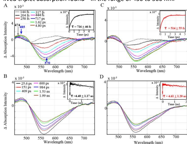
Fig. 2. OTA spectra of a solution of A. 0.3 mM AI-1 , C. 0.3 mM AI-2 in 0.93:0.07 \text{CH}_3\text{CN} :DMF upon light excitation at 355 nm between pump-probe delays from 144 fs up to 4.80 ps. Inset A,C. Kinetic decay profiles at \lambda = 485 nm after excitation at \lambda_{\text{exc}} = 355 nm illustrating the formation of the singlet excited state. OTA spectra of a solution of B. 0.3 mM AI-1 , D. 0.3 mM AI-2 in 0.93:0.07 \text{CH}_3\text{CN} :DMF upon light excitation at 355 nm between 25.6 ps and 1.99 ns. Inset B, D. Kinetic decay profiles at \lambda = 485 nm illustrating the intersystem crossing rate from the singlet to the triplet.
