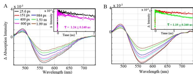
Fig. 3. OTA spectra of a complete photocatalytic system of A. 0.3 mM AI-1 , B. 0.3 mM AI-2 with 0.3 mM Fe catalyst, 30 mM BIH and 30 mM TEOA in 0.93:0.07 \text{CH}_3\text{CN} :DMF. Inset A,B. Quenching of the AI* singlet excited state by BIH to generate the reduced optically silent AI' reduced species.
