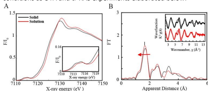
Fig. 1. A. Normalized Fe K-edge XANES of 1 mM of the FeQPYPY catalyst in solid (black) and a solution mixture of 0.93:0.07 CH 3 CN: DMF. Inset. Zoom-in of the pre-edge features B. Experimental Fourier transforms of k^2 -weighted Fe EXAFS of the FeQPYPY solid and solution complex (1 mM). Inset. Back Fourier transforms experimental (solid lines) and fitted (dashed lines) \text{Re}[\chi(k)] . Experimental spectra were calculated for k values of 2.118 to 13.443 Å -1 .
