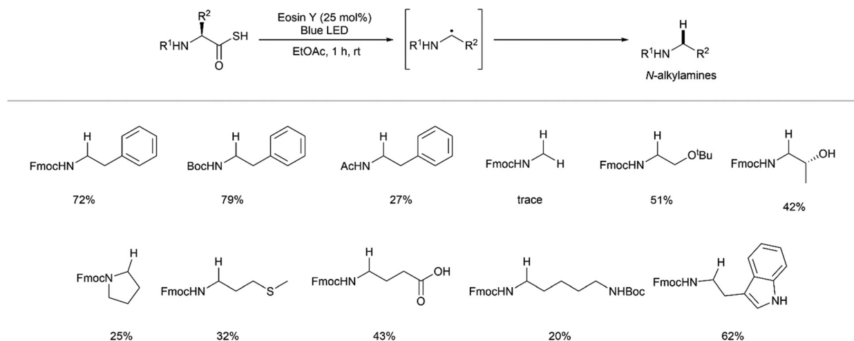
Fig. 27 Scope of dethiocarboxylation of amino acid thioacid derivatives under photoinitiation. 61
