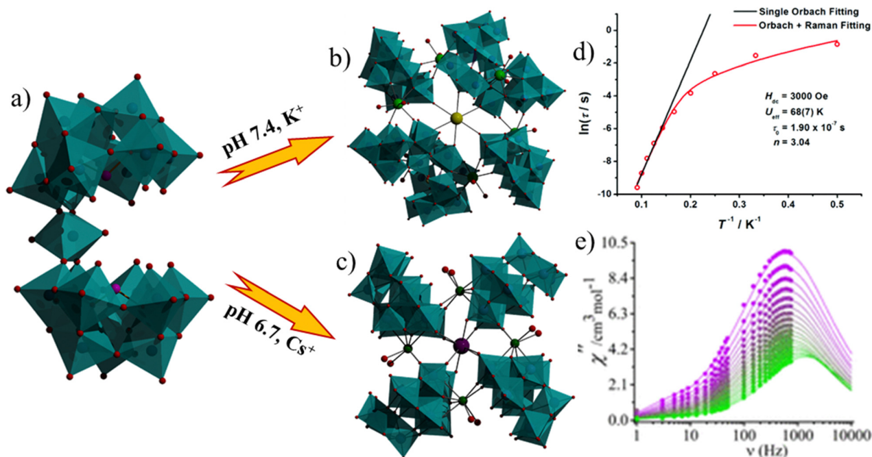
Fig. 3 The reaction conditions for the formation of [\text{K} \subset \{\alpha\text{AsW}_9\text{O}_{33}\}\text{Dy}(\text{H}_2\text{O})_2\text{O}_6]^{35-} (b) and [\text{Cs} \subset \{\text{Tb}_4(\text{H}_2\text{O})_8(\alpha\text{AsW}_9\text{O}_{33})_4\}]^{23-} (c) from [\text{As}_2\text{W}_{19}\text{O}_{67}(\text{H}_2\text{O})_{14}]^{4-} (a) and their corresponding magnetic relaxation plot (d) and frequency-dependent out-of-phase magnetic susceptibility plot (e). Color code: cyan octahedron \{\text{WO}_6\} , green Dy, red O, yellow K, violet Cs, pink As. Hydrogen atoms are omitted for clarity. Figures reprinted (adapted) with permission from ref. 97 and 101. Copyright (2022) American Chemical Society, and (2017) Royal Society of Chemistry, respectively.
