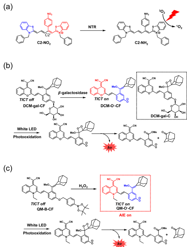
Fig. 11 TICT-based photosensitizers and chemiluminescent probes. (a) Photosensitizer; (b) chemiluminescent probes for \beta -galactosidase and light; (c) chemiluminescent probes for H 2 O 2 and light. The blue and red structures are the electron-donating and -accepting moieties, respectively.
