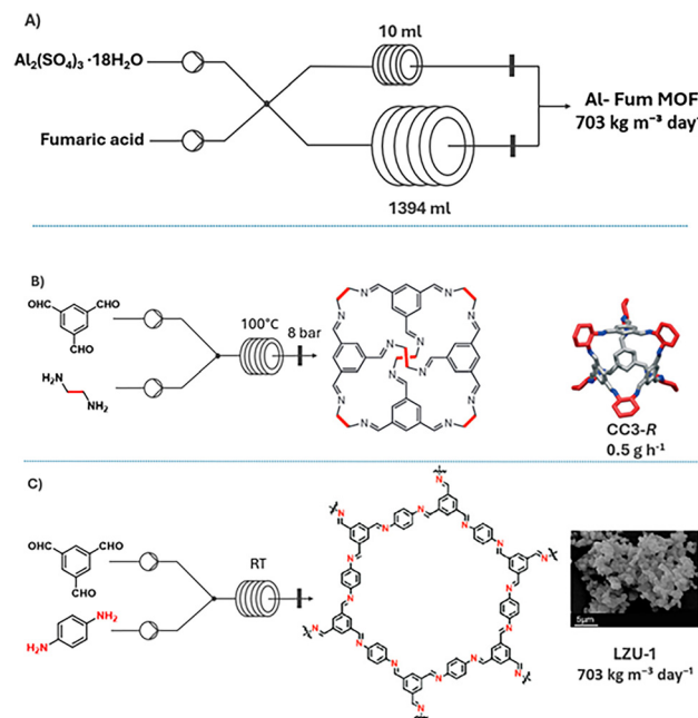
Fig. 2 Schematic representation of the formation of (A) Al-Fum MOF; (B) CC3-R and (C) LZU-1 in a flow reactor. Adapted with permission from ref. 74 (copyright 2016 Wiley-VCH), ref. 82 (copyright 2015 Royal Society of Chemistry) and ref. 78 (copyright 2015 American Chemical Society).
