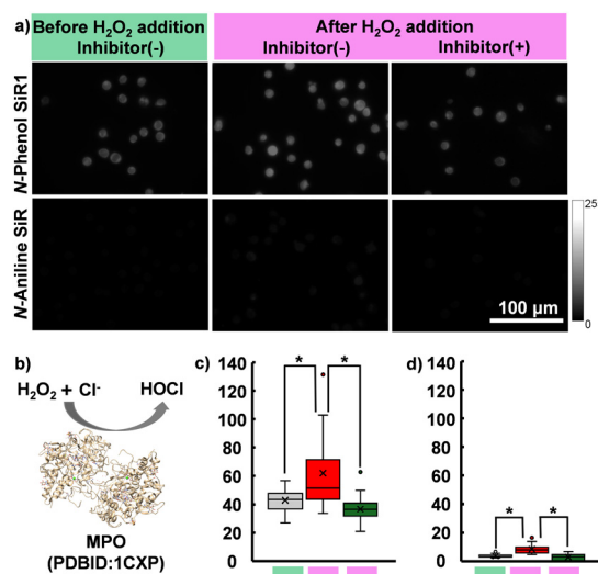
Fig. 4 Application of N -Phenol SiR1 and N -Aniline SiR for live-cell fluorescence imaging. (a) Fluorescence microscopic images of HL60 cells incubated with 1 μM N -Phenol SiR1 or N -Aniline SiR for 15 min, with or without the MPO inhibitor (4-ABHA), before and after addition of H 2 O 2 . (b) The MPO-based generation system of HClO from H 2 O 2 and chloride ions. (c) Fluorescence intensities of HL60 cells incubated with N -Phenol SiR1, from the fluorescence images of (a). (d) Fluorescence intensities of HL60 cells incubated with N -Aniline SiR, from the fluorescence images of (a). Error bars represent ± S.E. (n = 25). * Indicates p < 0.01 (Welch's t-test).
