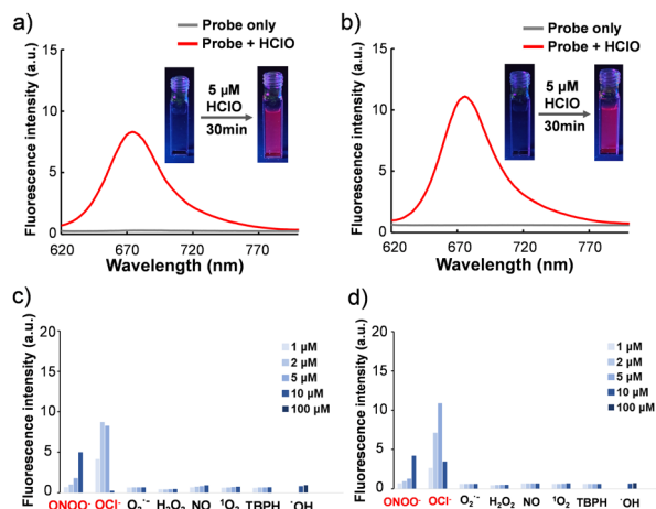
Fig. 3 (a) and (b) Fluorescence spectra of 1 μM (a) N -Phenol SiR1 and (b) N -Aniline SiR before (grey line) and after (red line) reaction with 5 μM HClO for 30 min. The excitation wavelength was 600 nm. (c) and (d) Fluorescence intensities at 672 nm of 1 μM (c) N -Phenol SiR1 and (d) N -Aniline SiR after reaction with various ROS. The fluorescence measurements were performed in PBS with excitation at 600 nm at 37 °C for 30 min. The slit widths for excitation and emission were both 5 nm. ONOO - : ONOONa; - OCl: NaOCl; O 2 •- : KO 2 ; H 2 O 2 : NOC 7 (0.5 eq.); 1 O 2 : EP-1; TBHP: t -BuOOH; • OH: 100 mM (or 1 M) H 2 O 2 and 10 μM (or 100 μM) FeCl 2 (Fenton reaction).
