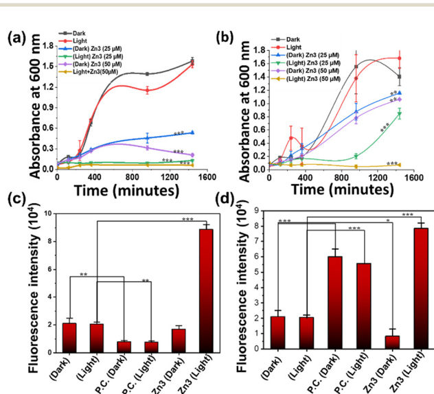
Fig. 3 (a) and (b) Kinetics growth curve of Zn3 -treated E. coli (a) and B. subtilis (b) under light and dark conditions. (c) and (d) In-cell ROS production in (c) E. coli and (d) B. subtilis induced by Zn3 (50 \mu\text{M} ) under light and dark conditions.
