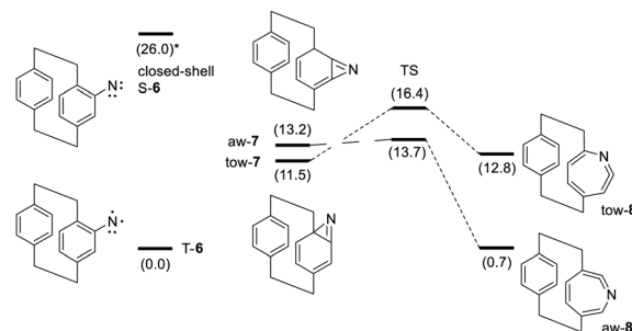
Scheme 2 Potential energy diagram of the rearrangement products of 6 based on zero-point corrected energies ( \Delta E_{\text{ZPC}} , in kcal mol -1 ) computed at the (U)B3LYP-d3bj/def2TZVP level of theory. The singlet energy was computed for the closed-shell structure S-6.
