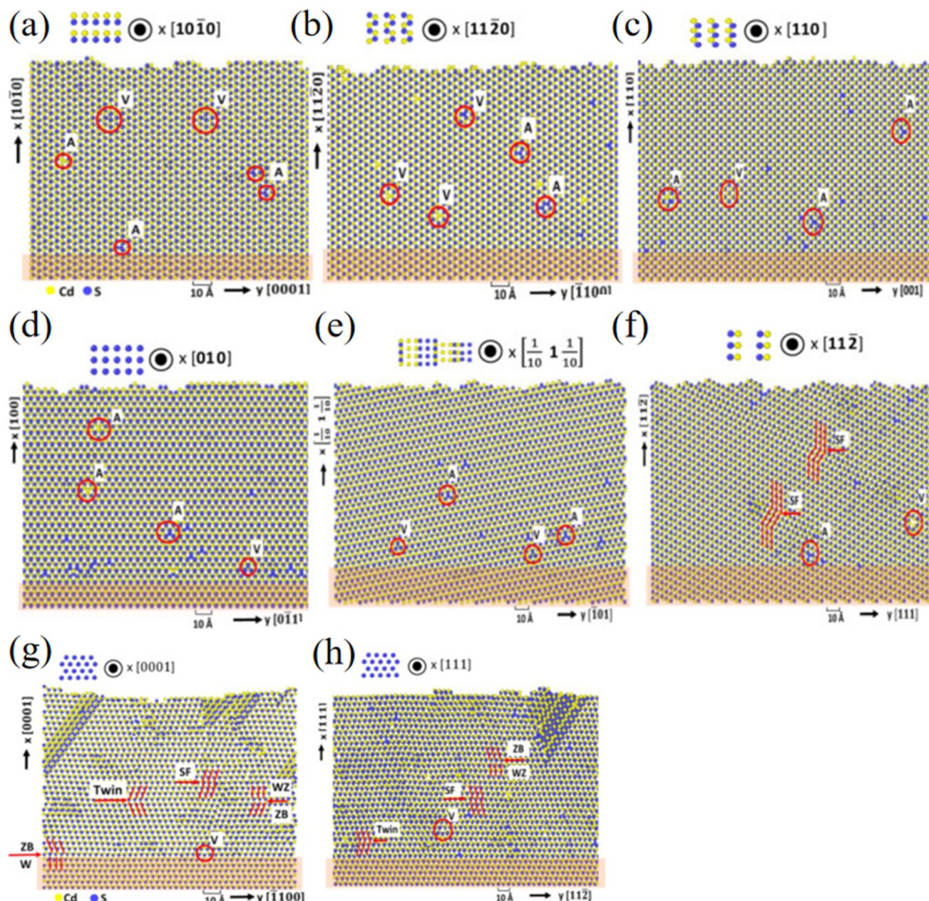
Fig. 7 Atomistic visualizations of MD simulations for CdS homoepitaxial growth along (a) [10\bar{1}0] WZ, (b) [11\bar{2}0] WZ, (c) [110] ZB, (d) [010] ZB, (e) [\frac{1}{10}\frac{1}{10}] ZB, (f) [11\bar{2}] ZB, (g) [0001] WZ and (h) [111] ZB directions. Shaded regions represent the initial substrate (copyright from Elsevier, Journal of Crystal Growth). 51
