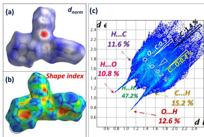
Fig. 3 Hirshfeld surfaces analysis shown in: d_{\text{norm}} (a) and shape index (b) mode for compound I, Computed fingerprint plots (c).
