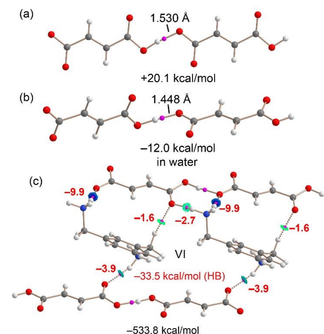
Fig. 25. QTAIM (BCPs in pink and bond path as dashed bonds) and NCIplot (RDG = 0.5, \rho cut-off = 0.04 a.u., color scale -0.035 a.u. \leq (\text{sign}\lambda_2)\rho \leq 0.035 a.u. for the H-bonded anion...anion dimer in the X-ray (a) and optimized (b) geometries. (c) QTAIM analysis of a hexameric fragment of VI. The energies of the assemblies and those derived from potential energy densities (in red) are indicated in kcal/mol.
