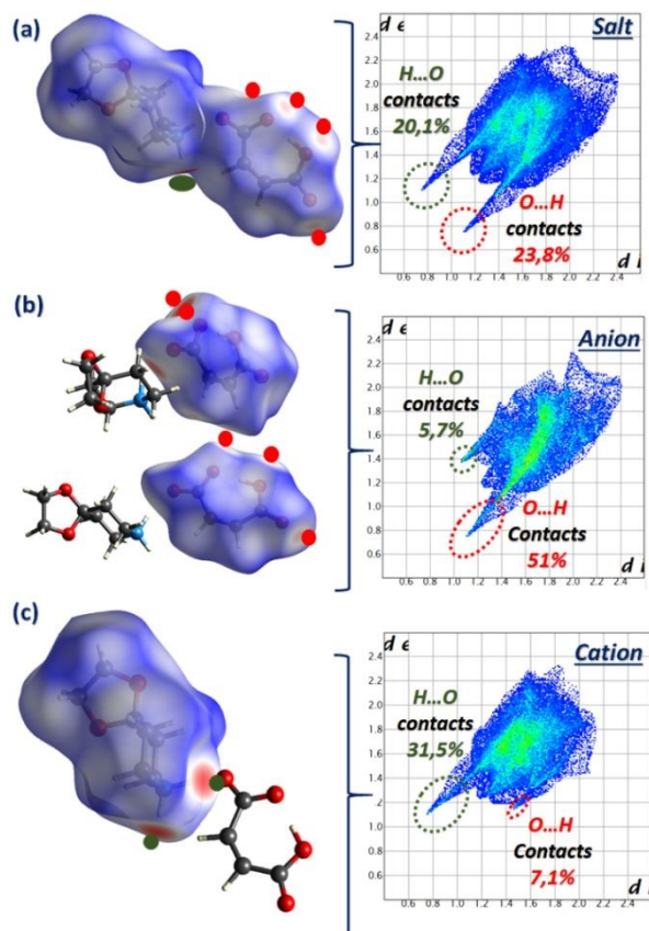
Fig. 7 Hirshfeld surface mapped over d_{\text{norm}} mode with their associated finger print plots of (a) 1,4-DAD/MA salt and its (b) anion and (c) cation.
