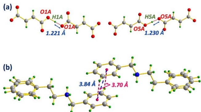
Fig. 4 Intramolecular H-bonding interactions formed between anions (a), Presentation of C-H... \pi and \pi ... \pi stacking between N-Benzylphenethylaminium cations (b).
