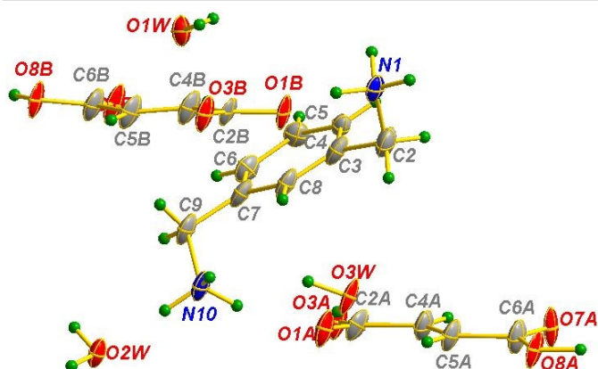
Fig. 15 Asymmetric unit of m -Xylylenediamine/Fumaric acid-Trihydrate salt (VI) with atom-labeling scheme.
