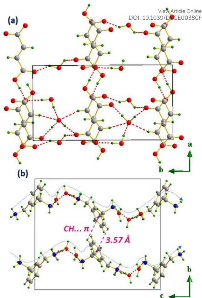
Fig. 16 Molecular packing of anions (a) and cations (b) separately in m -Xylylenediamine/Fumaric acid-Trihydrate salt (VI).
