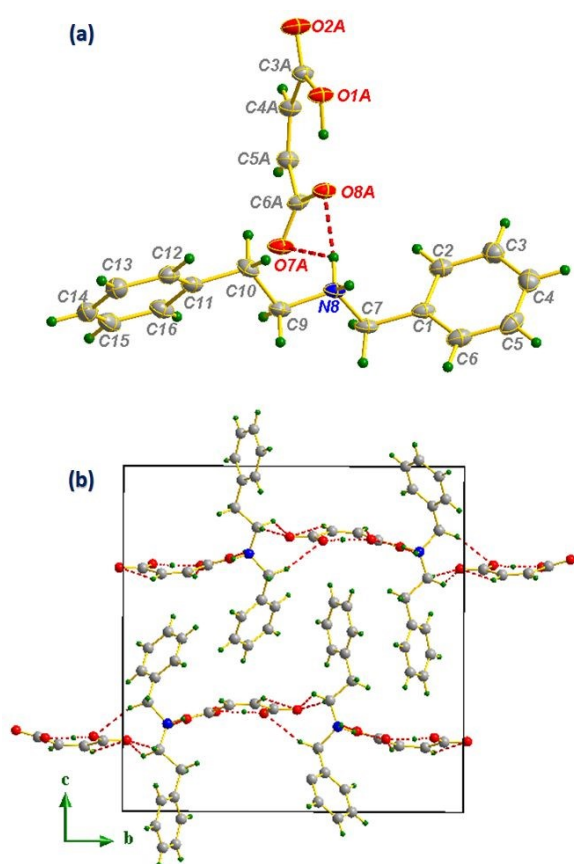
Fig. 1 Ortep representation of compound I (Ellipsoids are drawn at 45% probability level) (a), projection along the (b,c) plane (b).
