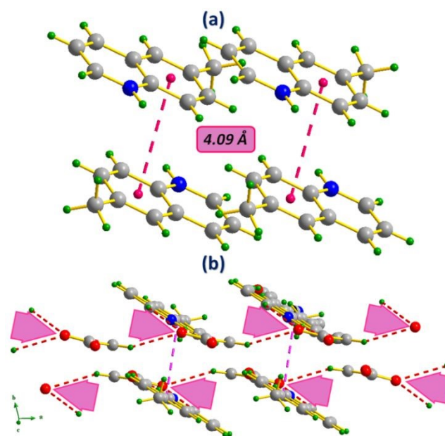
Fig. 13 Representation of 6-Methylquinolines \pi\cdots\pi arrangement (a), Combination of hydrogen bonding and \pi -stacking interactions (b).
