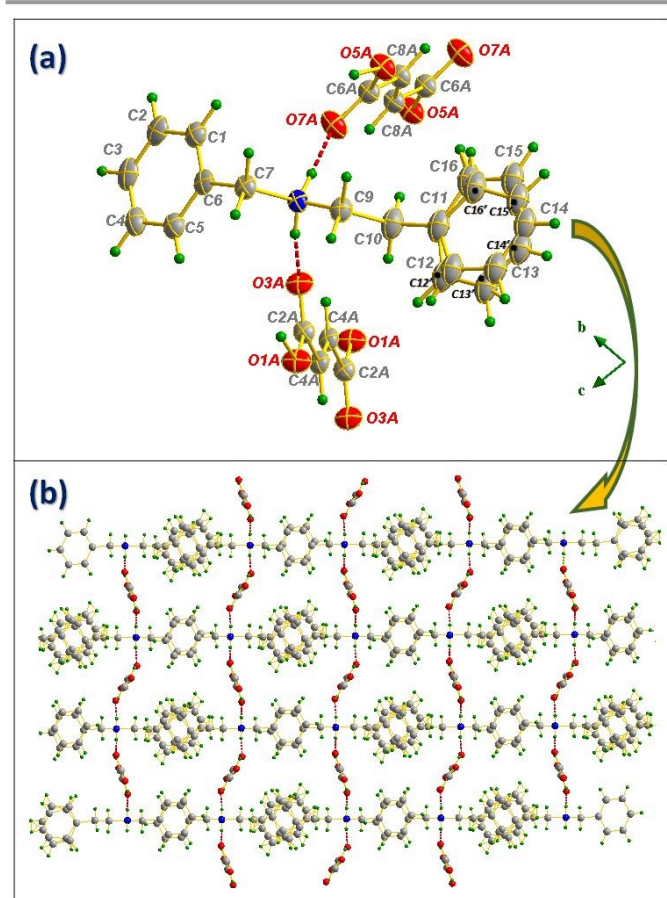
Fig. 6 Asymmetric unit of compound III (a), Projection of the structure along the (\vec{a}, \vec{c}) plane (b) marking the formation of R_3^2(8) and R_1^2(4) supramolecular synthons between anion and cation (c), Intra- and intermolecular S(7) and R_3^2(7) interaction motif formed between MAs (d).
