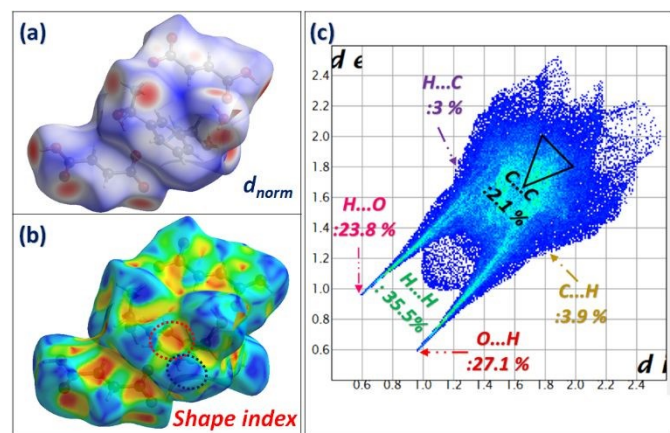
Fig. 18 Hirshfeld surface analysis in d_{\text{norm}} mode (a), Shape index (b) and the calculated fingerprint plots (c) of m-Xylylenediamine/Fumaric acid-Trihydrate salt (IV)
