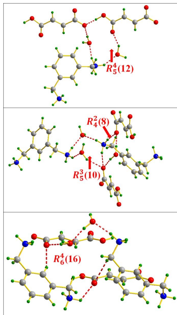
Fig. 21 supramolecular synthons made up as the result of \text{FA}\cdots\text{MXDA}\cdots\text{water} interaction in m-Xylylenediamine/Fumaric acid-Trihydrate salt (IV)
