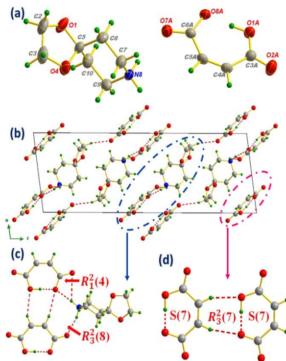
Fig. 6 Asymmetric unit of compound III (a), Projection of the structure along the (\vec{a}, \vec{c}) plane (b) marking the formation of R_3^2(8) and R_1^2(4) supramolecular synthons between anion and cation (c), Intra- and intermolecular S(7) and R_3^2(7) interaction motif formed between MAs (d).
