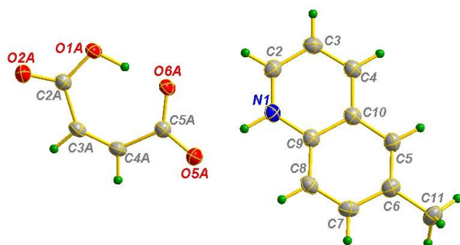
Fig. 11 Asymmetric unit representation of 6-Methylquinoline /Maleic acid salt.
