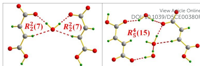
Fig. 19 supramolecular synthons formed via \text{FA}\cdots\text{water} inter-molecular interaction in m-Xylylenediamine/Fumaric acid-Trihydrate salt (IV)
