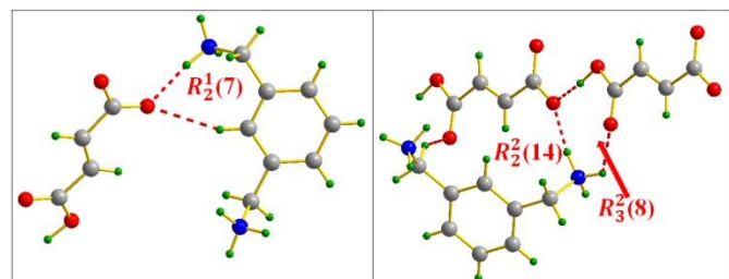
Fig. 20 \text{FA}\cdots\text{MXDA} intermolecular interaction motifs in m-Xylylenediamine/Fumaric acid-Trihydrate salt (IV)
