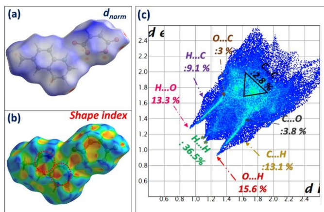
Fig. 14 d_{\text{norm}} mode (a), Shape index (b), Calculated fingerprint plots of 6-Methylquinoline/Maleic acid salt (c).
