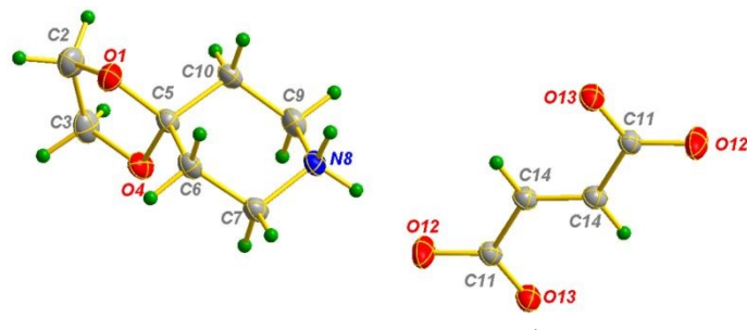
Fig.8 Ortep representation of 1,4-Dioxa-8-azaspiro(4.5)decane/Fumaric acid salt.
