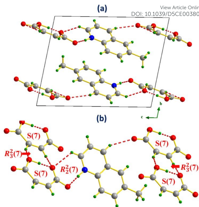
Fig. 12 Projection of the compound V structure along the (\vec{b}, \vec{c}) plane (a), Intra- and intermolecular interaction motifs formed in compound V (b).
