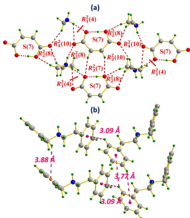
Fig. 2 Intra- and intermolecular interaction motifs formed in salt I (a), C-H... \pi interaction distances (b).
