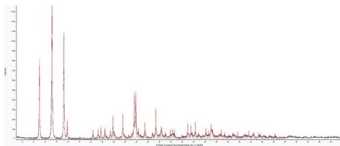
Figure 4: PXRD of the new AgSD-NO 3 (black) compared with theoretical pattern (red).
