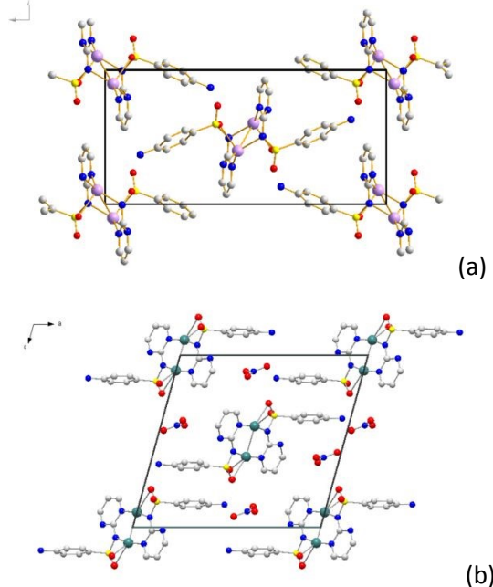
Figure 5: Supramolecular packing of AgSD-NO 3 depicting the formation of (a) chains along the b -axis and (b) the hexagonal array in the a - c plane.
