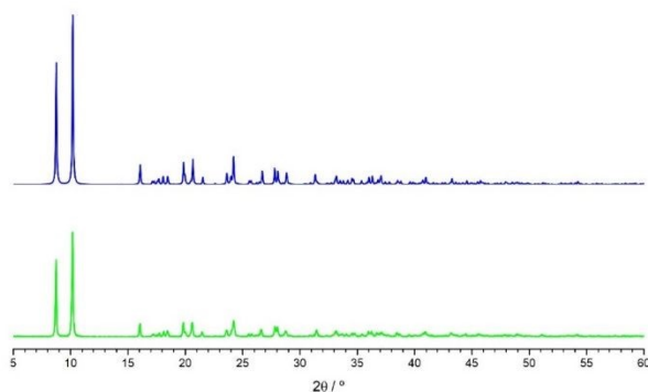
Figure 2: PXRD diffractograms collected at \lambda (Cu K\alpha_1 ) = 1.54056 Å of AgSD reported as SULPMS (green) experimentally obtained by the LAG method and simulated (blue).
