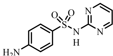
Figure 1 - Chemical Structure of Sulfadiazine (SD).
