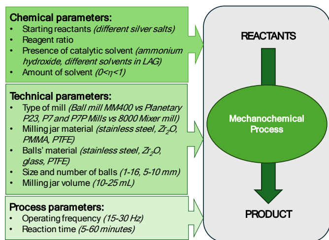
Chart 1: Schematic representation of selected parameters that may influence mechanochemical reactions. Image adapted from reference 24 with the permission of Royal Society of Chemistry.
