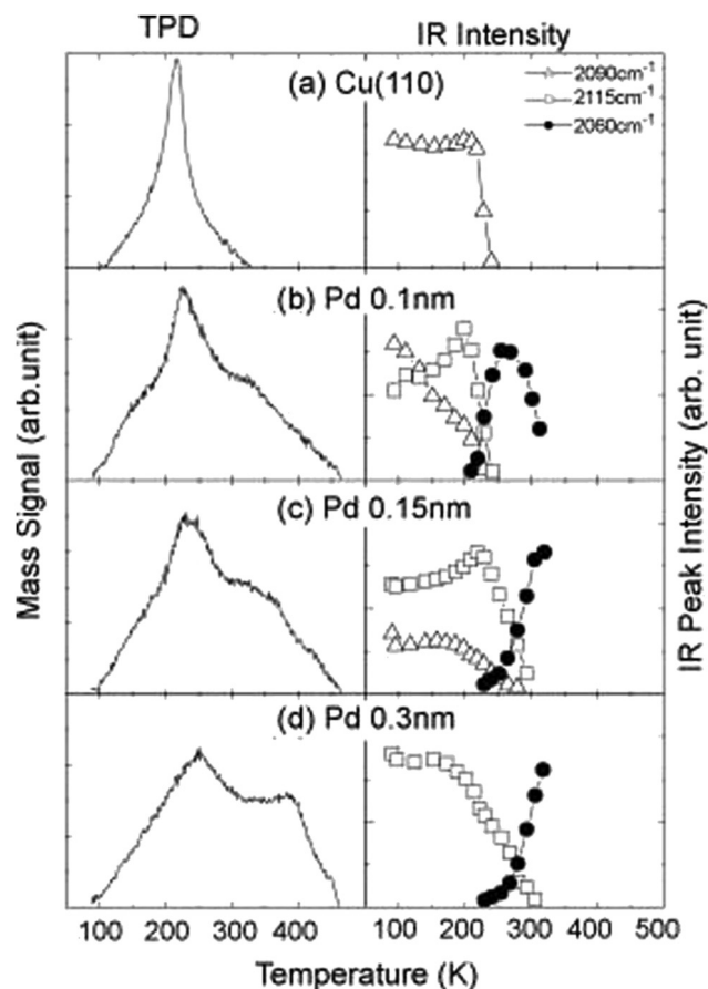
Fig. 3 The TPD spectra (left) and RARS peak intensity changes (right) with elevating the substrate temperature for the 1.0-Langmuir (L)-CO exposed surfaces: (a) clean Cu(110), (b) 0.1-nm-thick-, (c) 0.15-nm-thick-, and (d) 0.3-nm-thick-Pd/Cu(110). Heating rate for TPD measurements: 3 \text{ K s}^{-1} . 112 Reprinted with permission from ref. 112. Copyright 2008 Elsevier.
