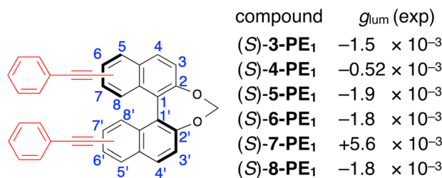
Fig. 1 Summary of our recent study 17 on methylene-linked binaphthol derivatives ( S )- 3-PE 1 to ( S )- 8-PE 1 with phenylethynyl (PE) groups at from 3,3' to 8,8' positions on the binaphthyl backbone and their dissymmetry ( g_{lum} ) values for CPL.
