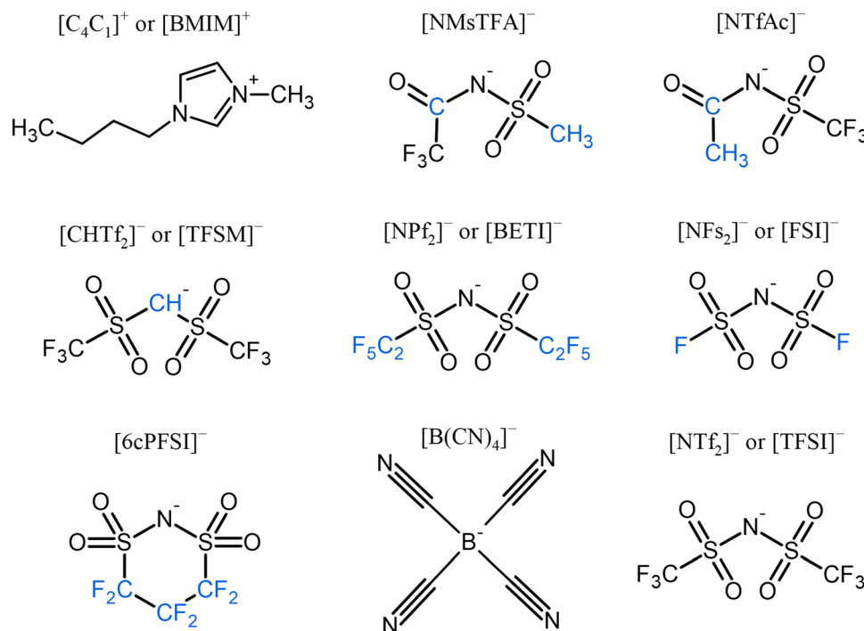
Fig. 1 Molecular structure of the cation [BMIM] + and the anions of the studied ILs. The [TFSI] - anion is included for comparison purposes and the chemical modifications in the anions are highlighted in blue color.
