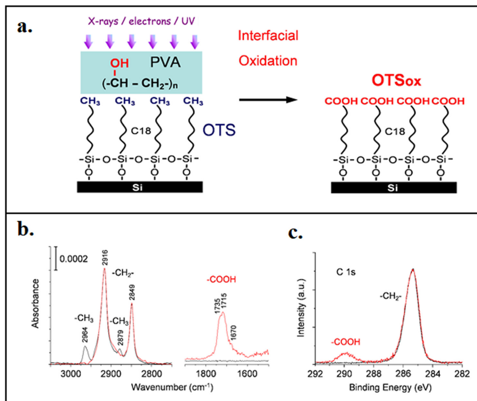
Fig. 6 Interfacial beam-induced chemical transformation. (a) Schematics of the molecular structures in interfacial solid-phase oxidation of an OTS/Si monolayer to OTS ox /Si, using a thin PVA film as an oxidation reagent. Irradiation means (X-ray, electrons, UV) used to activate the process are indicated. The bare OTS ox surface is revealed upon ex situ removal of the PVA film. (b) Quantitative Brewster angle FTIR spectra of the pristine OTS/Si monolayer (black) and the irradiated monolayer after removal of the PVA film (red). (c) XPS C 1s line, as recorded from a pristine OTS/Si monolayer, before depositing the PVA film (black), and from the X-ray irradiated PVA-coated OTS/Si, after complete removal of the irradiated PVA film (red). Peak heights in panel c are normalized for visual convenience. Note the combined XPS and FTIR indications for COOH formation upon XPS irradiation, while the CH 3 signal in FTIR vanishes. Taken from ref. 94.
