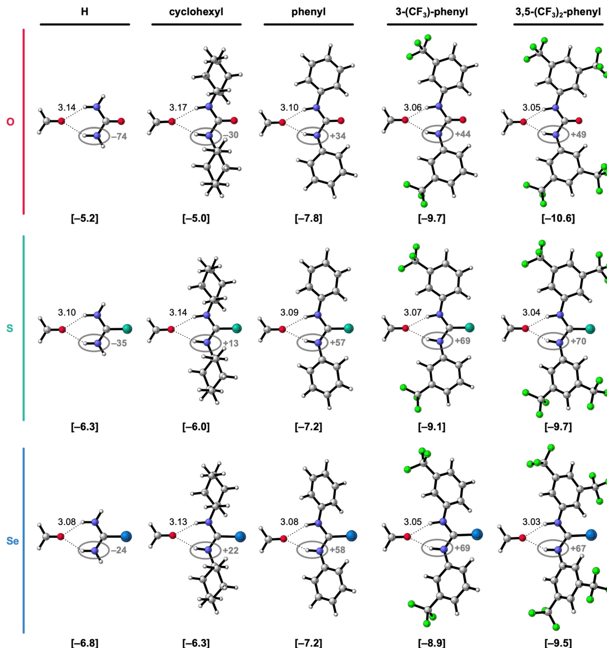
Fig. 3 Equilibrium hydrogen-bonded complexes of formaldehyde with 1,3-disubstituted X-urea derivatives ( X = O, S , or Se ; R^1 = R^3 ). 17 The equilibrium hydrogen-bond ( O \cdots (H)N ) distances (in Å) are indicated and the hydrogen-bond energies \Delta E (in \text{kcal mol}^{-1} ) are shown below the structures between square brackets. The total Voronoi deformation density (VDD) atomic charge Q_{NH} of the NH groups (in milli-electrons) of the isolated X-urea in the geometry of the hydrogen-bonded complex is highlighted in grey. Color code of the ball-and-stick structures: H = white; C = grey; N = dark blue; O = pink; F = green; S = turquoise; Se = light blue.
