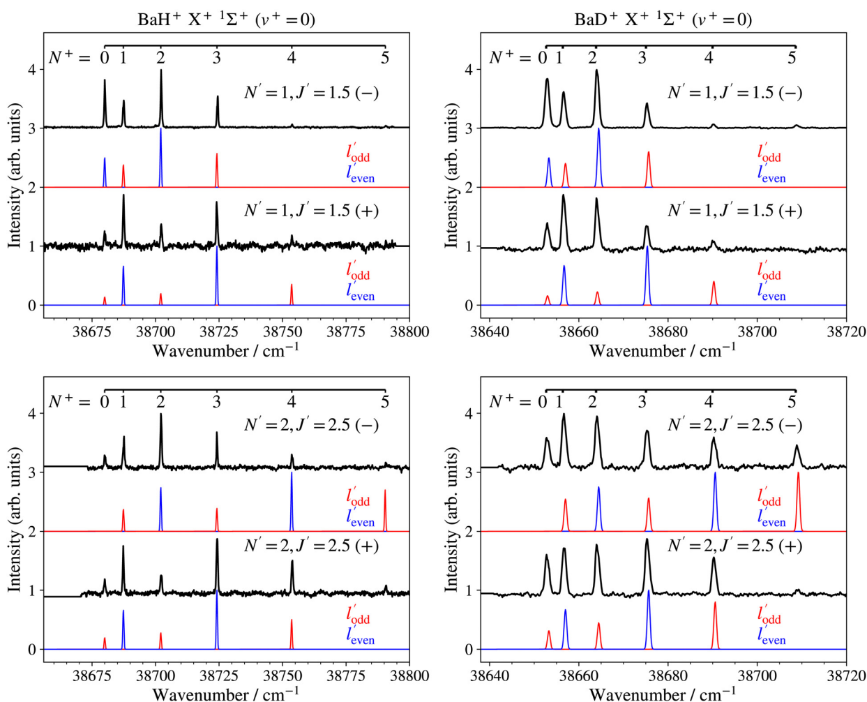
Fig. 8 High-resolution PFI-ZEKE-PE spectra of the \text{X}^+ \text{1}\Sigma^+ ( v^+ = 0, N^+ ) \leftarrow \text{E}^2\Pi_{1/2} [ v' = 0, N', J', (-/+) ] ionising transitions of BaH and BaD. The assignment bars give the values of the rotational quantum N^+ . The blue and red traces correspond to intensity contributions from different configurations of the \text{E}^2\Pi_{1/2} state and expected for ionisation out of molecular orbitals of dominant \ell = 1 ( \ell' even) and 2 ( \ell' odd) characters, respectively, in single-centre expansions of the orbitals.
