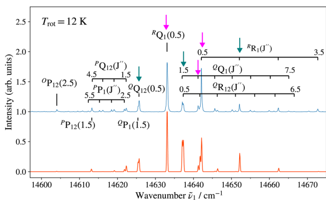
Fig. 3 (1 + 1') R2PI spectrum of the E 2 Π 1/2 (ν' = 0)–X 2 Σ + (ν'' = 0) transition of 138 BaH acquired with an ionisation-laser wavenumber \tilde{\nu}_2 of 26 878.72 cm -1 with assignment of the highest-intensity ΔN ΔJ F 1 (F 2 )(J'') lines. Bottom: Spectrum calculated for a rotational temperature of 12 K and convoluted with a Gaussian lineshape function with a full width at half maximum of 0.25 cm -1 . The lines marked by vertical arrows (pink, aqua) are those used to prepare intermediate states of well-defined parity (–, +) to characterise the photoionisation dynamics.
