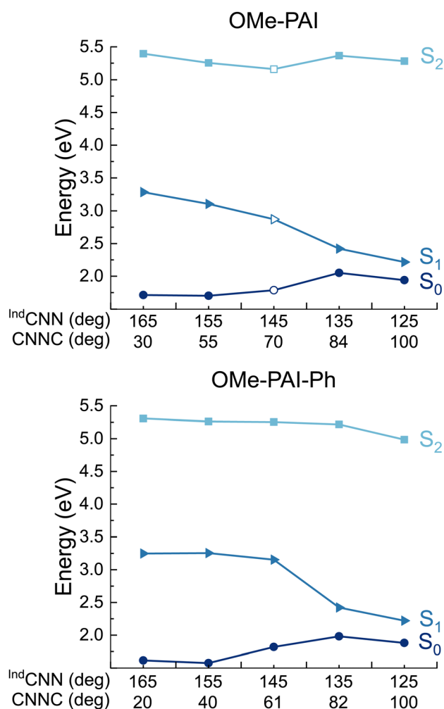
Fig. 4 First three singlet potential energy curves along the ^{\text{Ind}}\text{CNN} -CNNC seam (marked in white in Fig. 3) for OMe-PAI and OMe-PAI-Ph. For OMe-PAI-Ph this is the same \text{S}_0 seam as the blue in Fig. 5. For OMe-PAI, four indole-side relaxed geometries are extracted from the ^{\text{Ind}}\text{CNN} -CNNC \text{S}_0 surface, and an open circle energy average is added to assist the interpretation. CAM-B3LYP/6-311G(d,p)-D3BJ/PCM(MeCN).
