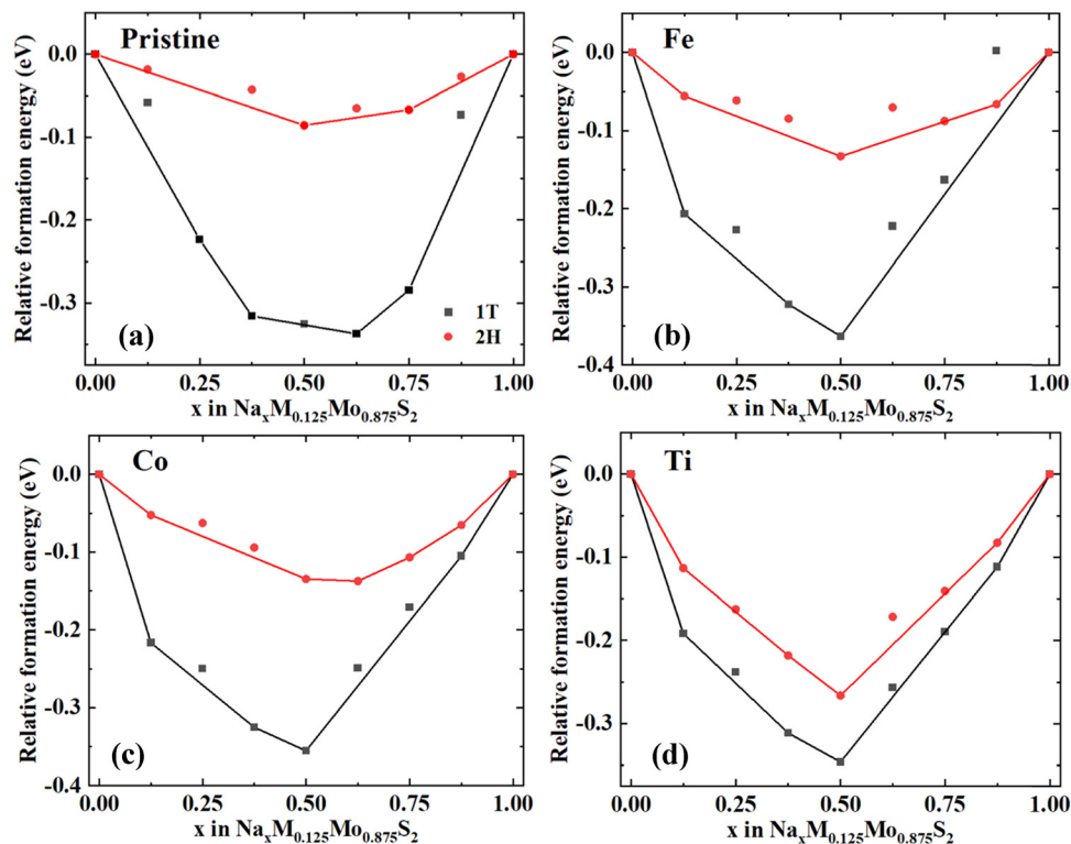
Fig. 6 Convex hull of the 1T and 2H phase (a) pristine, (b) Fe, (c) Co, and (d) Ti doping MoS 2 structures.
