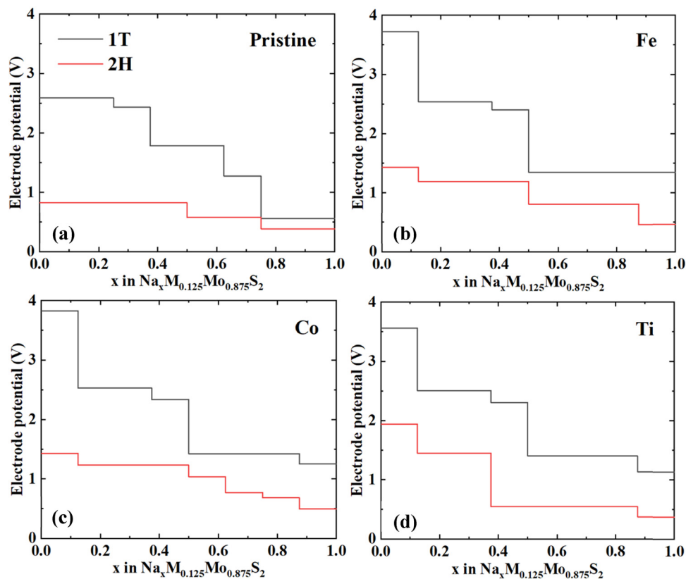
Fig. 7 OCV curves of 1T and 2H phase (a) pristine, (b) Fe, (c) Co, and (d) Ti doping MoS 2 structures.
