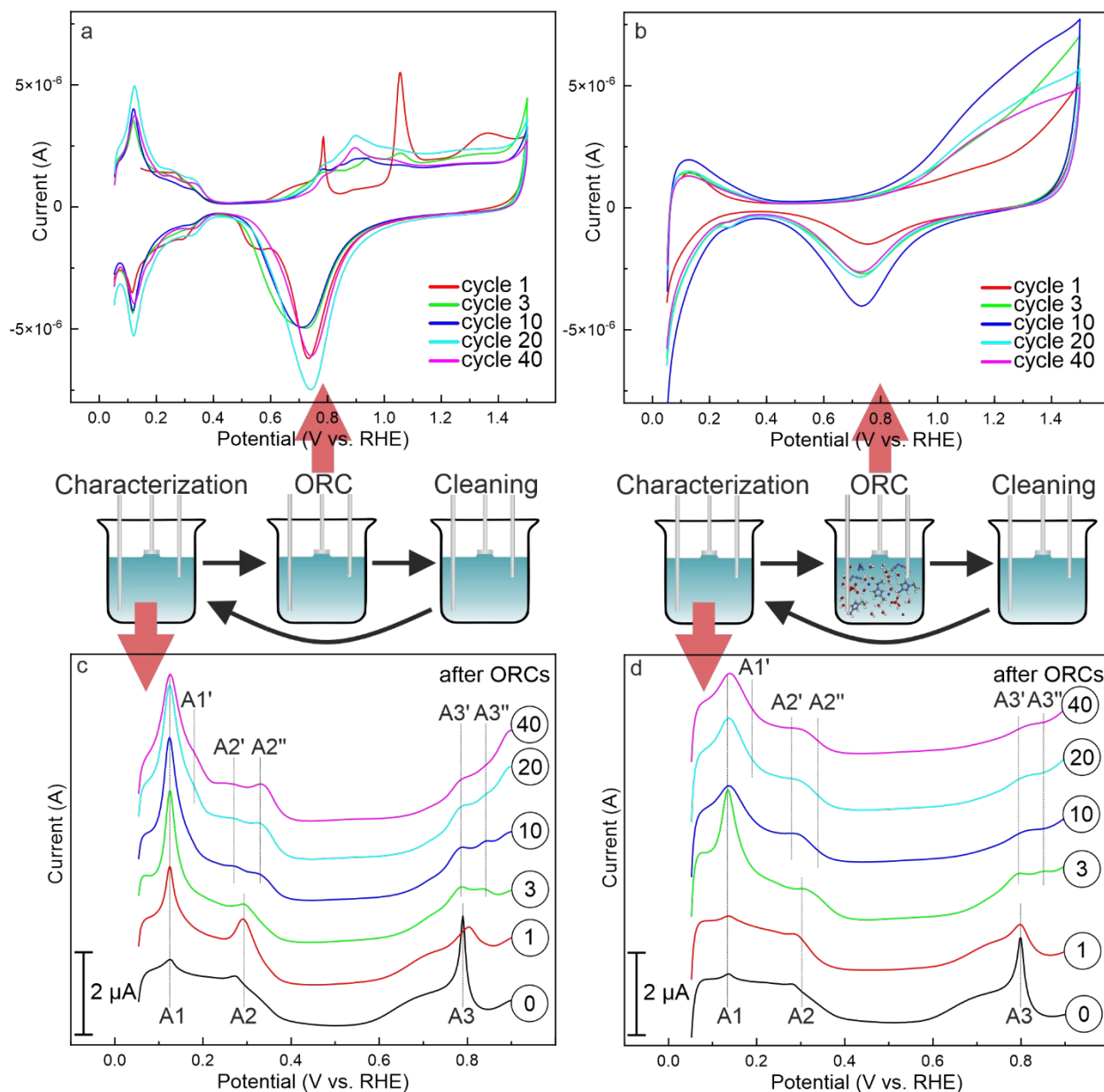
Figure 2: Cyclic voltammograms of Pt(111) during ORCs (0.05 – 1.5 V RHE , 50 mV·s -1 ) in the absence (a) and presence (b) of 1 M [C 2 C 1 Im][OTf]. Corresponding characterization CVs (0.05 – 0.9 V RHE , 50 mV·s -1 ) measured after ORCs in absence (c) and presence (d) of IL in blank electrolyte only (0.1 M HClO 4 ). An additional cleaning step was performed between the ORCs and the characterization.
