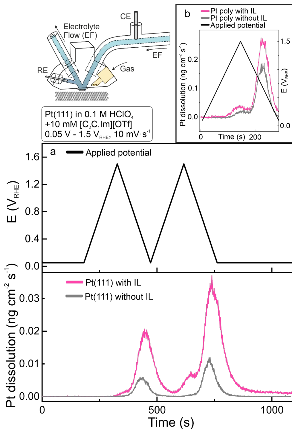
Figure 3: (a) Online ICP-MS dissolution profiles for two consecutive CVs from Pt(111) in 0.1 M HClO 4 in the absence and presence of 10 mM [C 2 C 1 Im][OTf]. (b) Corresponding reference experiment of polycrystalline Pt. Applied electrochemical potential window 0.05 - 1.5 V RHE , scan rate 10 mV·s -1 .
