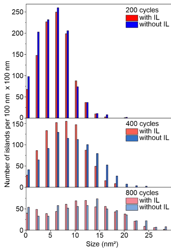
Figure 6: Size distribution histogram of nanoislands in EC-STM images from Figure 5. The corresponding values are summarized in Table 1.
