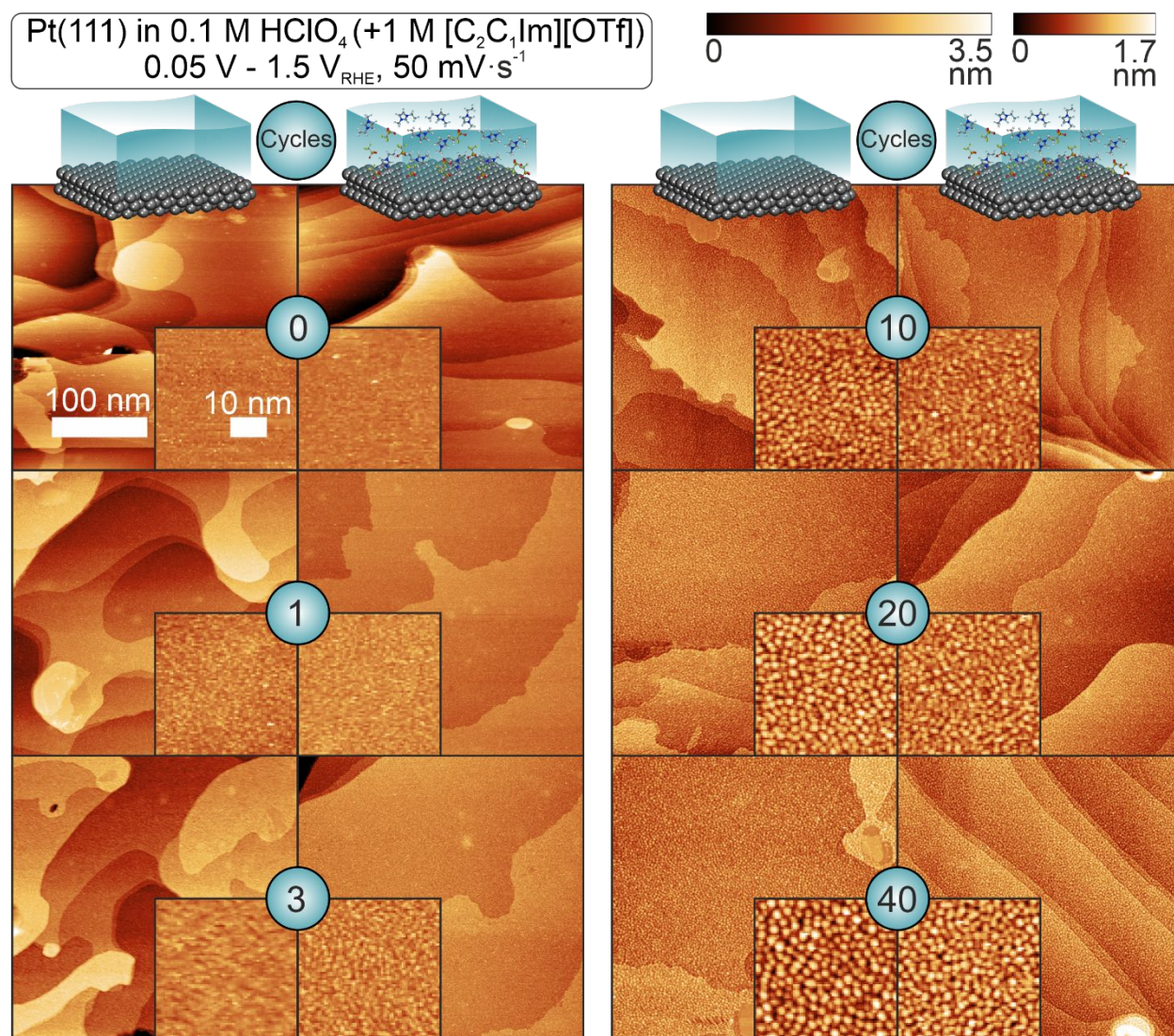
Figure 4: EC-STM images ( U_{\text{bias}} 0.4 V, I_t 0.2 - 1 nA) before and after the initial oxidation-reduction cycles (0.05 - 1.5 V RHE , 50 mV·s -1 ) in the absence (left) and presence (right) of 1 M [C 2 C 1 Im][OTf]. Supporting electrolyte was 0.1 M HClO 4 .
