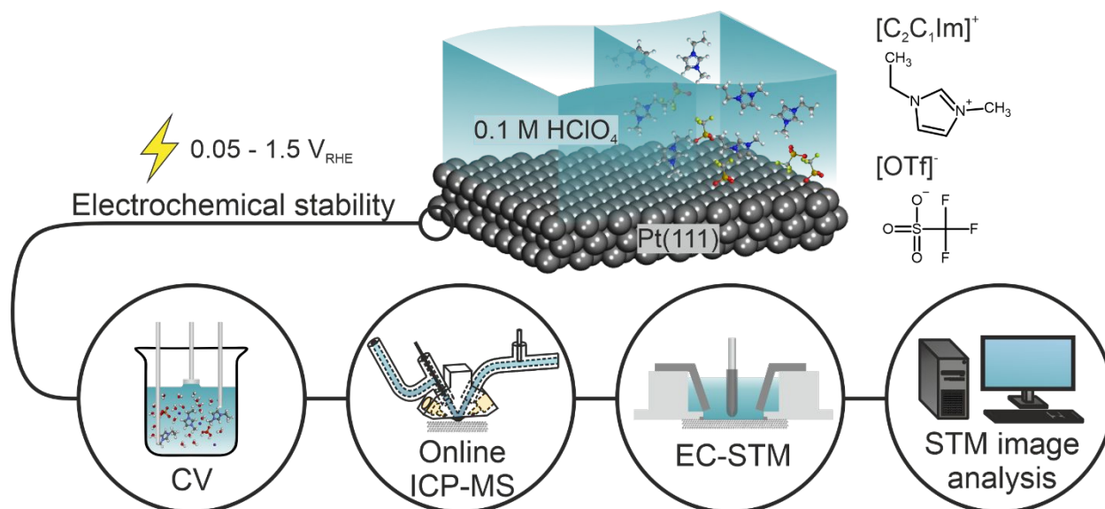
Figure 1: Electrochemical system studied in this work. Stability of Pt(111) in 0.1 M HClO 4 in absence and presence of the ionic liquid [C 2 C 1 Im][OTf]. We probe the electrochemical stability of the system applying CV, online ICP-MS, EC-STM and using an algorithmic pattern recognition approach to analyze STM images.
