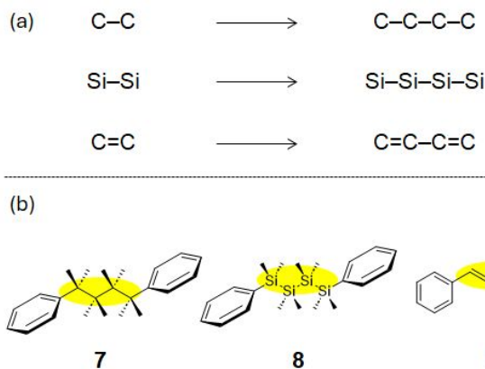
Fig. 6 (a) Expansion of linkage chain. (b) Chemical structures of 7–9.
