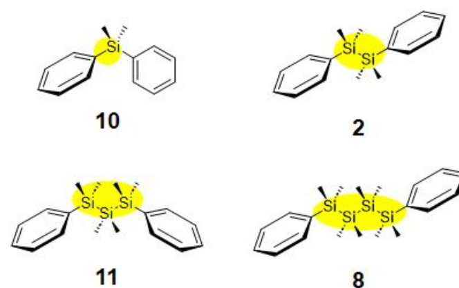
Fig. 9 Structures of \alpha,\omega -diphenyloligosilanes to study the effect of silicon length.
