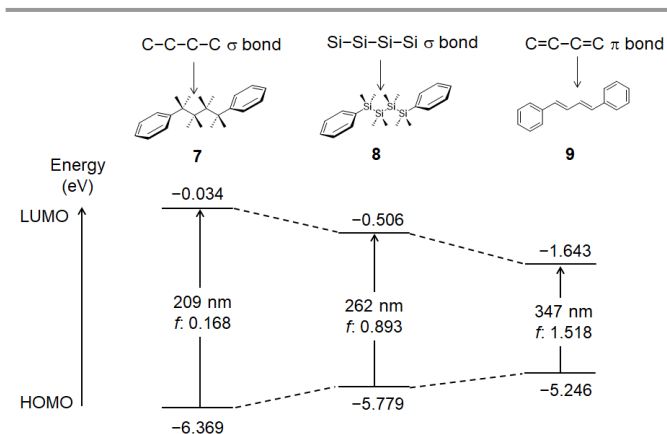
Fig. 8 HOMO and LUMO energy levels, HOMO–LUMO energy gaps, calculated absorption wavelengths, and oscillator strengths of 7–9 .
