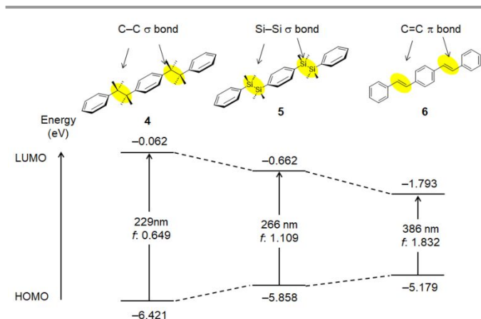
Fig. 5 HOMO and LUMO energy levels, HOMO-LUMO energy gaps, calculated absorption wavelengths, and oscillator strengths of 4–6.
