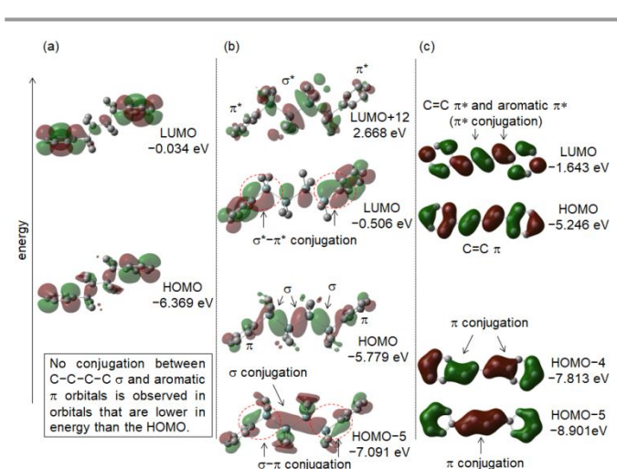
Fig. 7 Molecular orbitals and energy levels of 7–9. (a) LUMO and HOMO of 7. (b) LUMO+12, LUMO, HOMO, and HOMO-5 of 8. (c) LUMO, HOMO, HOMO-4, and HOMO-5 of 9. Hydrogen atoms are omitted for clarity. The isovalue is set to 0.03.
