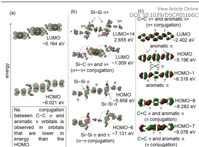
Fig. 4 Molecular orbitals and energy levels of 4 – 6 . (a) LUMO and HOMO of 4 . (b) LUMO+14, LUMO, HOMO, and HOMO–6 of 5 . (c) LUMO, HOMO, HOMO–1, HOMO–5, HOMO–6, and HOMO–7 of 6 . Hydrogen atoms are omitted for clarity. The isovalues are set to 0.03.
