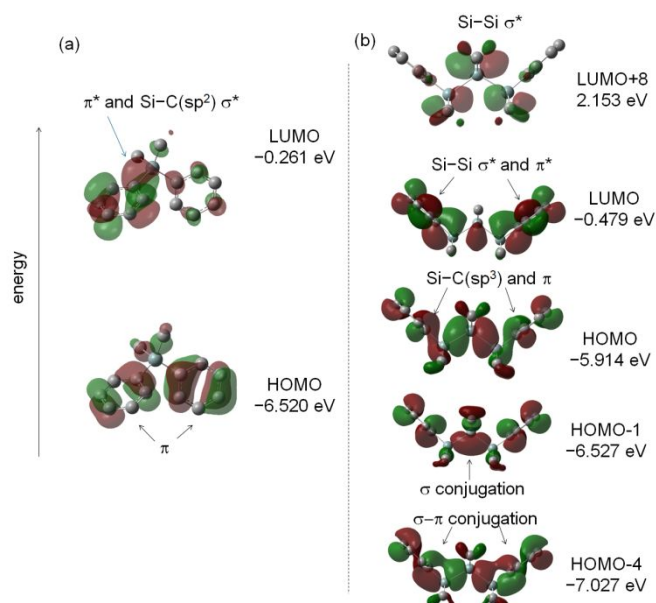
Fig. 10 Molecular orbitals of 10 and 11 . (a) LUMO and HOMO of 10 . (b) LUMO+8, LUMO, HOMO, HOMO-1, and HOMO-4 of 11 . Hydrogen atoms are omitted for clarity. The isovalues are set to 0.03.
