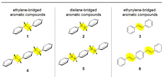
Fig. 1 Chemical structures of 1–6.
