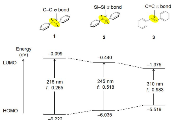
Fig. 3 HOMO and LUMO energy levels, HOMO–LUMO energy gaps, calculated absorption wavelengths, and oscillator strengths of 1–3 .
