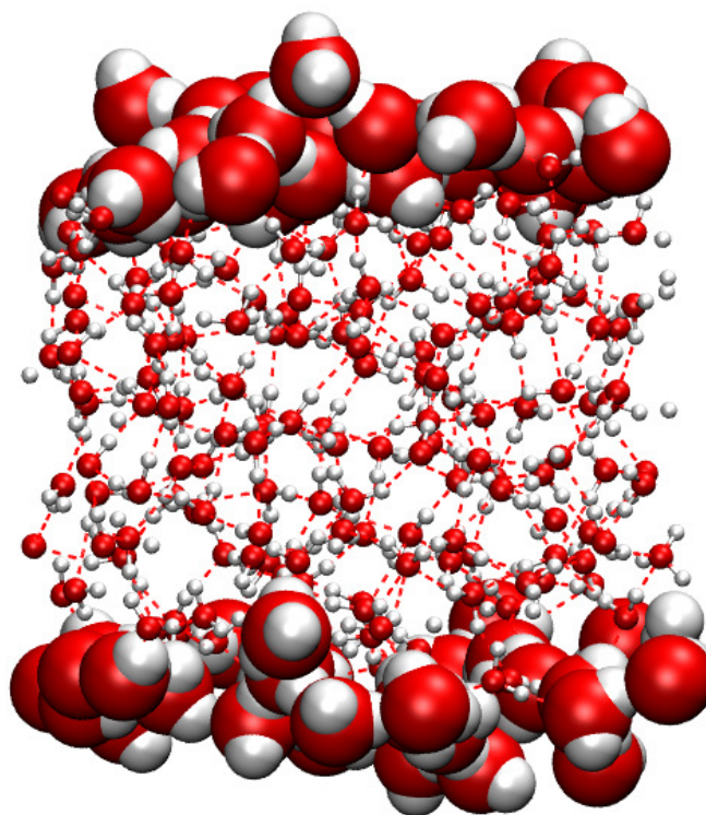
Figure 1: A representative snapshot of the water-air interface obtained from AIMD simulation in presence of static field of strength 0.01 \text{ V/\AA} . The topmost layer identified using ITIM algorithm.
