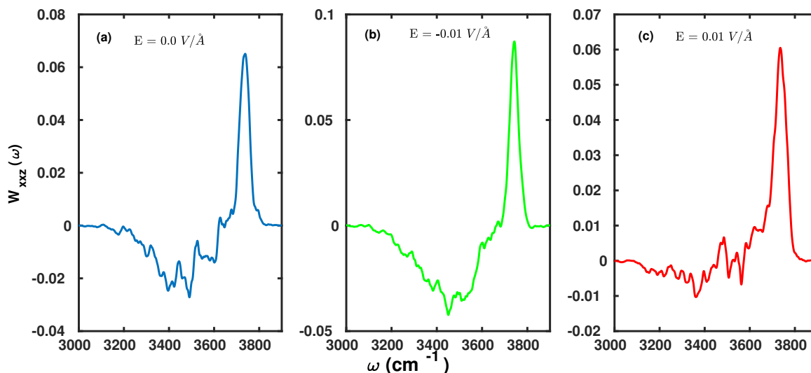
Figure 3: Time averaged vibrational spectral density of the OH modes of the interfacial molecules in the presence of external field of strength (a) 0.00, (b) -0.01, and (c) +0.01 V/Å respectively.
