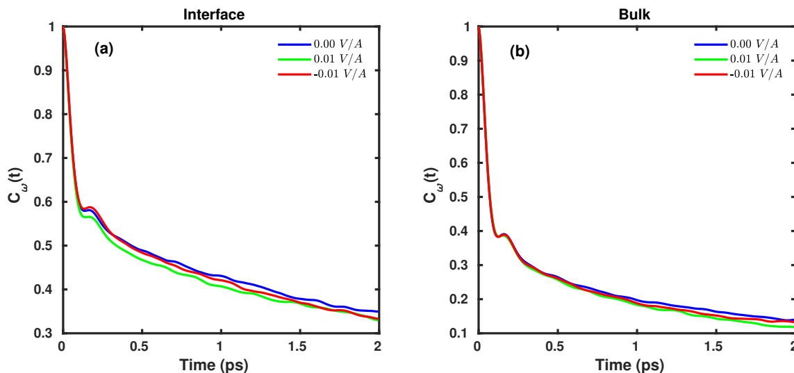
Figure 5: Time-dependent decay of the FTICFs of OH modes of water molecules for the field strength of 0.00, 0.01 and -0.01 V/Å at the (a) water-air interface and (b) in bulk.
