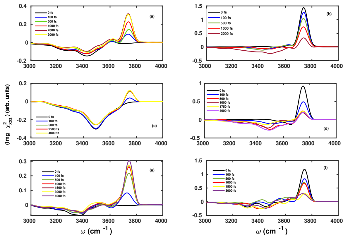
Figure 6: TD-vSFG spectra of the air-water interface in the presence of an external electric field of strength 0.00 V/Å for (a) hydrogen-bonded OH modes and (b) free OH modes, and -0.01 V/Å for (c) hydrogen-bonded OH modes and (d) free OH modes, and +0.01 V/Å for (e) hydrogen-bonded OH modes and (f) free OH modes.
