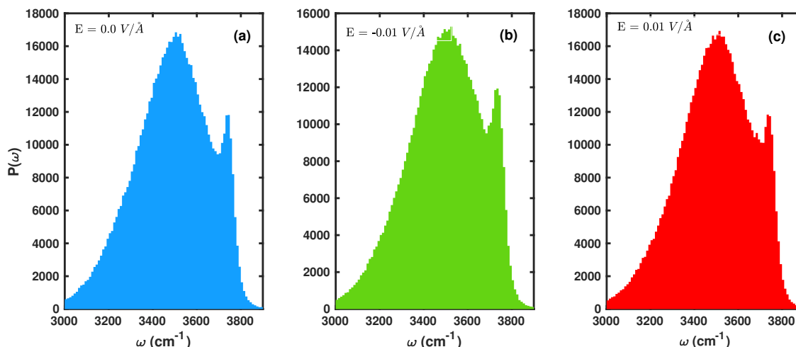
Figure 4: Time-averaged vibrational frequency distribution of the OH modes of the water molecules at the water-air interface in presence of external field of strength (a) 0.00, (b) -0.01 and (c) +0.01 V/Å respectively.
