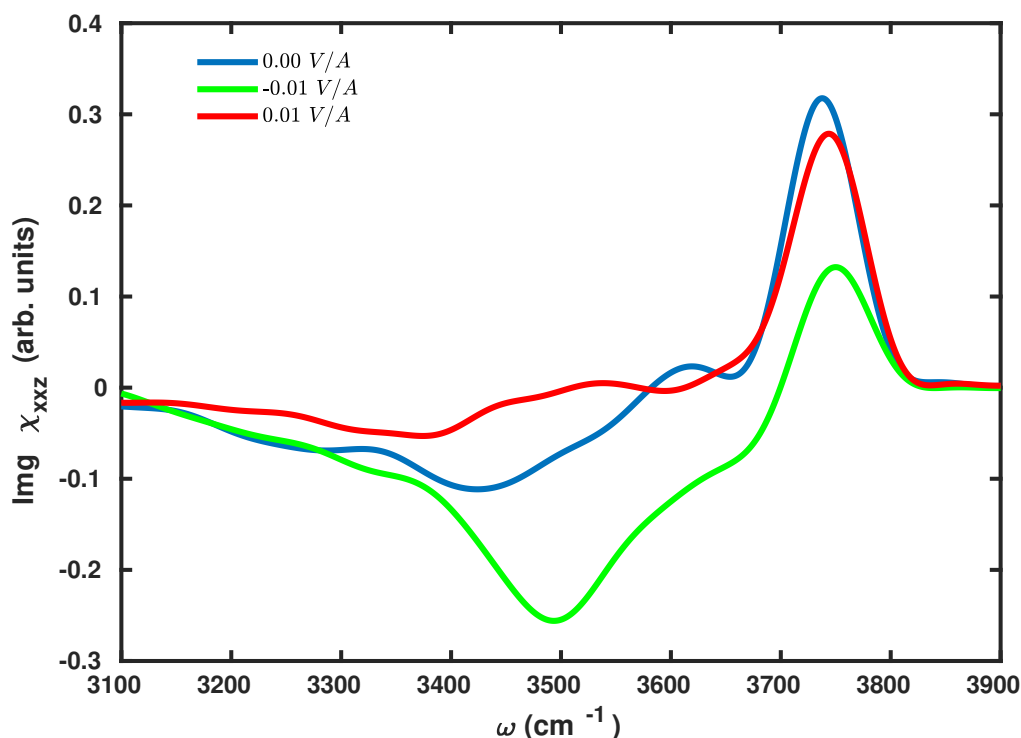
Figure 2: The Imaginary xxz component of the second order susceptibility ( \chi_{xxz}^2 ) of the OH mode of water molecules at the water-air interface in the presence of external field of strength \pm 0.01 V/Å and in the ambient conditions.
