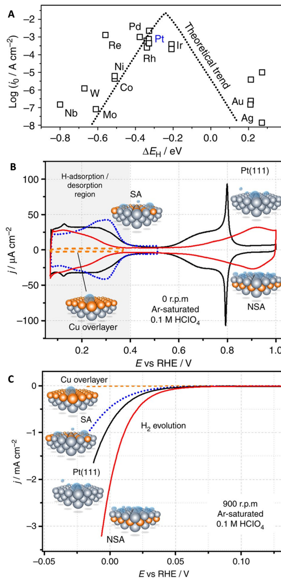
Fig. 5 (A) Experimental HER activity in terms of exchange current density ( \log(i_0) ) for various metal surfaces against the calculated \ast H chemisorption energy ( \Delta E_H ). The results of a simple theoretical kinetic model are also depicted as a dotted line. (B) CVs and (C) RDE voltammetry for Cu overlayer, Pt(111), surface alloy (SA), and NSA in Ar-saturated 0.1 M HClO_4 , illustrating the correlation between HER activity and the position of Cu atomic layers relative to the topmost Pt layer. Reproduced with permission from ref. 107 Copyright 2016, Nature Publishing Group.
