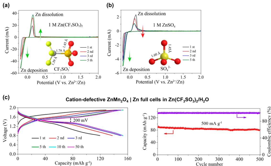
Fig. 52 Cyclic voltammograms of the Zn plating/stripping in (a) 1 M \text{Zn}(\text{OTf})_2 and (b) 1 M \text{ZnSO}_4 solutions. (c) Galvanostatic charge and discharge curves at 50 \text{mA g}^{-1} and (d) long-term cycling performance of carbon-coated cation-defective \text{ZnMn}_2\text{O}_4 | Zn full cells in 3 M \text{Zn}(\text{OTf})_2/\text{H}_2\text{O} at 500 \text{mA g}^{-1} . 595 Reprinted with permission from Journal of the American Chemical Society .
