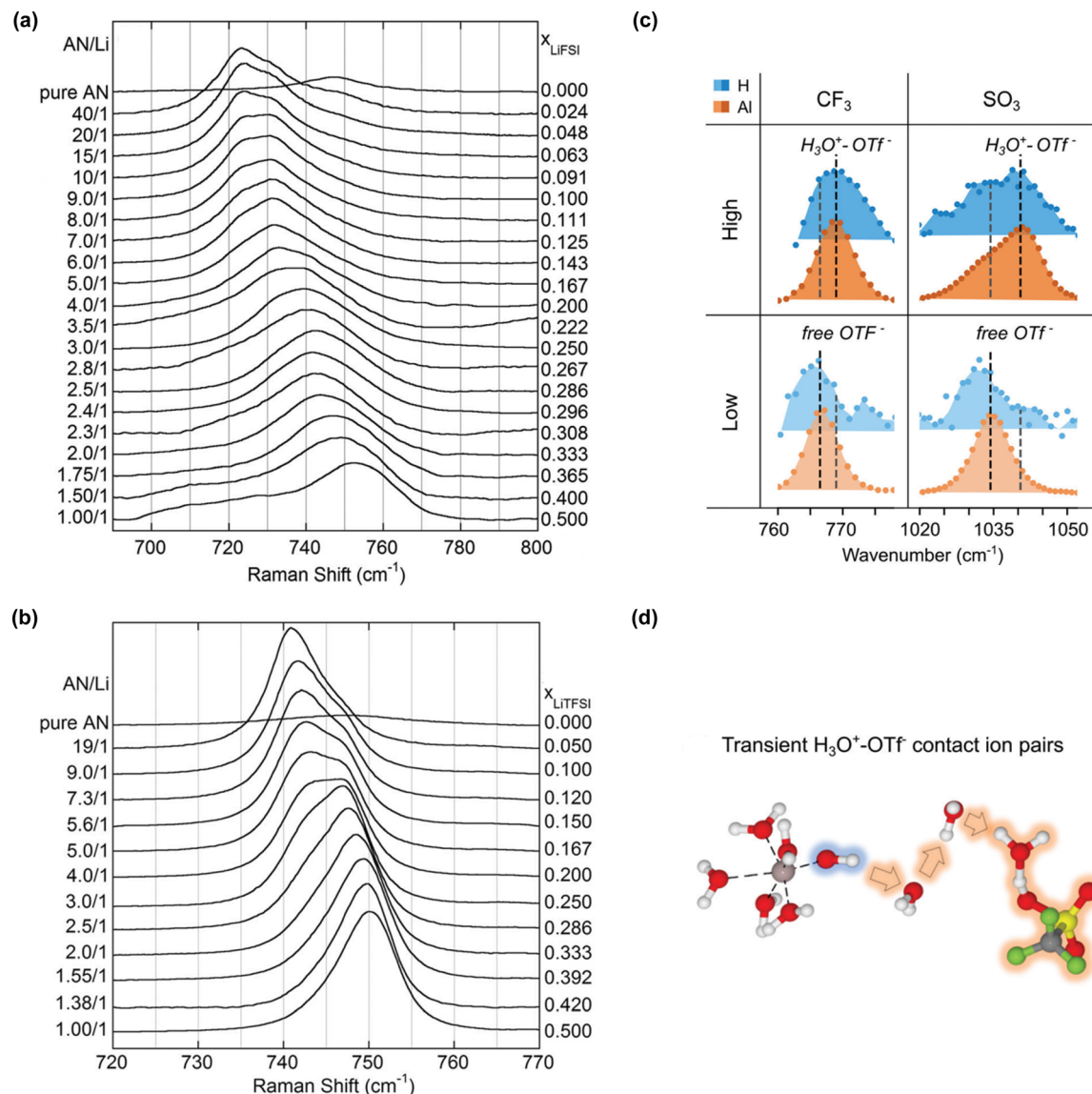
Fig. 43 Representative Raman spectra of (a) FSI −421 and (b) TFSI −425 anions in nonaqueous electrolytes, illustrating variational bands of the anion in LiFSI/acetonitrile and LiTFSI/acetonitrile electrolytes. (c) Raman spectra of CF 3 and SO 3 vibrational bands in Al(OTf) 3 and HOTf solutions at different salt concentrations, labelled "low" and "high" in the figure. 424 (d) Schematic of H 3 O + –OTf − ion pairing. 424 Reprinted with permission from Journal of The Electrochemical Society (a) and (b) and Energy & Environmental Science (c) and (d).
