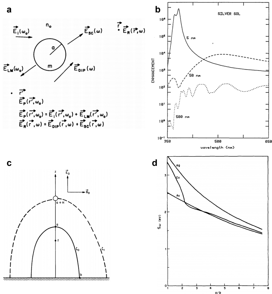
Fig. 8 (a) Schematic view of electric fields near sphere of radius a and refractive index m . At the incident frequency \omega_o there are the incident, Lorenz–Mie, and primary fields, E_i(\omega_o) , E_{LM}(\omega_o) , and E_p(r, \omega_o) . At the shifted frequency \omega there are the dipole, scattered, and Raman fields, E_{DIP}(\omega) , E_{SC}(\omega) , and E_R(r, \omega) , where r' and r are the positions of the dipole and observer, respectively. (b) Calculated enhancement for a 1010\text{ cm}^{-1} Raman band of molecules that are adsorbed on Ag spheres of radii 5, 50, and 500 nm. Reproduced from ref. 80 with permission. Copyright 1980 Optica publishing. (c) Geometry of surface protrusion. The semimajor axis is a and the semi minor axis is b . The spheroid surface is \zeta = \zeta_0 and that surface passing through the molecule is \zeta = \zeta_1 . (d) Energy of surface plasmons for Ag, Cu, and Au as a function of the aspect ratio of the spheroid. Reproduced from ref. 81 with permission. Copyright 1980 AIP publishing.
