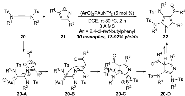
Scheme 7 Gold-catalyzed formal [3+2] annulation of yndiamides 20 with isoxazoles 21 .
