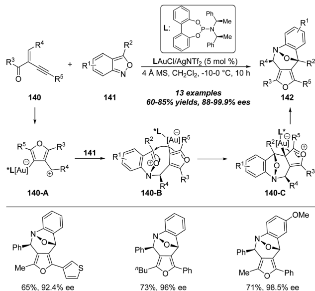
Scheme 45 Gold-catalyzed asymmetric formal [4+3] annulation of enynes 140 with anthranils 141 .
