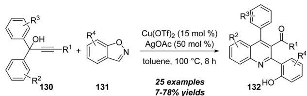
Scheme 42 Copper-catalyzed [4+2] annulation of propargylic alcohols 130 and benzod[1]isoxazoles 131 .
