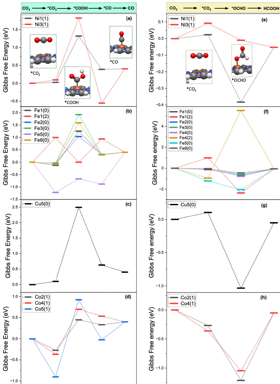
Fig. 3 Gibbs free energy diagram for the CO 2 R to CO according to the PCET mechanism on (a) Ni-POR, (b) Fe-POR, (c) Cu-POR, and (d) Co-POR. Gibbs free energy diagram for the CO 2 R to HCOOH according to the PCET mechanism on (e) Ni-POR, (f) Fe-POR, (g) Cu-POR, and (h) Co-POR. Calculations conducted at the B3LYP/LANL2DZ/COSMO level of theory. Values in eV.
