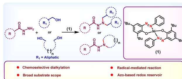
Scheme 1 Selective catalytic N,N -dialkylolation of acyl hydrazides using aliphatic alcohols.
