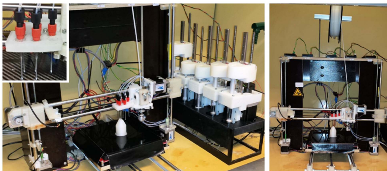
Fig. 18 Photographic view of a Prusa i3 RepRap printer modified into a robotic platform set-up with a 3D-printed reaction for the automated synthesis of ibuprofen Reproduced with permission. Copyright 2016, Beilstein Journal of Organic Chemistry . 157
