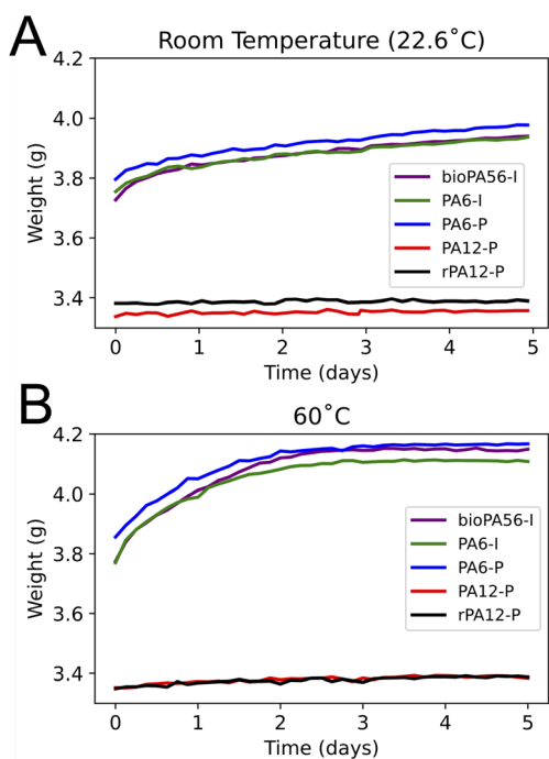
Fig. 5 Evolution of the weight of the polyamide specimens at (A) room temperature and (B) 60 °C.
