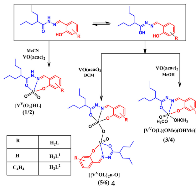
Scheme 1 Schematic of the synthesis of the complexes.
