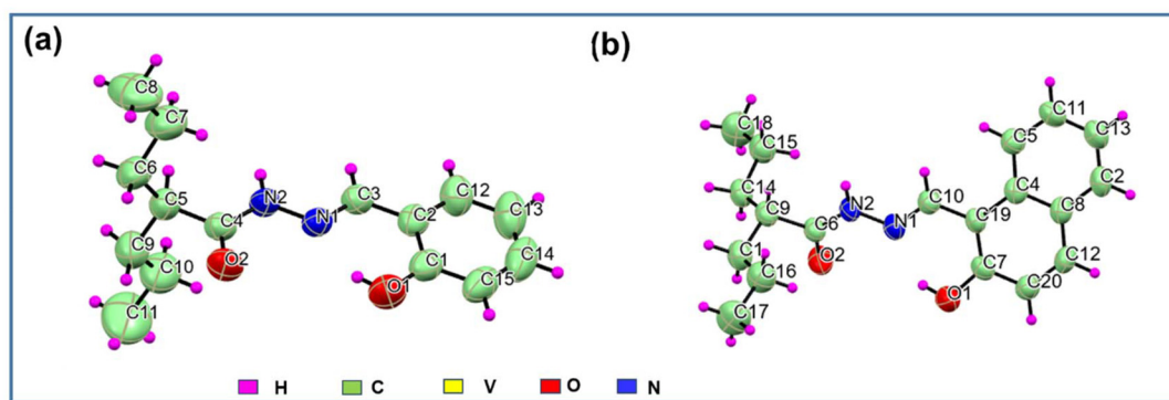
Fig. 1 ORTEP diagram (50% ellipsoid probability) and atom-numbering scheme for ligands (a) \text{H}_2\text{L}^1 (the disordered part has been omitted for clarity) and (b) \text{H}_2\text{L}^2 .
