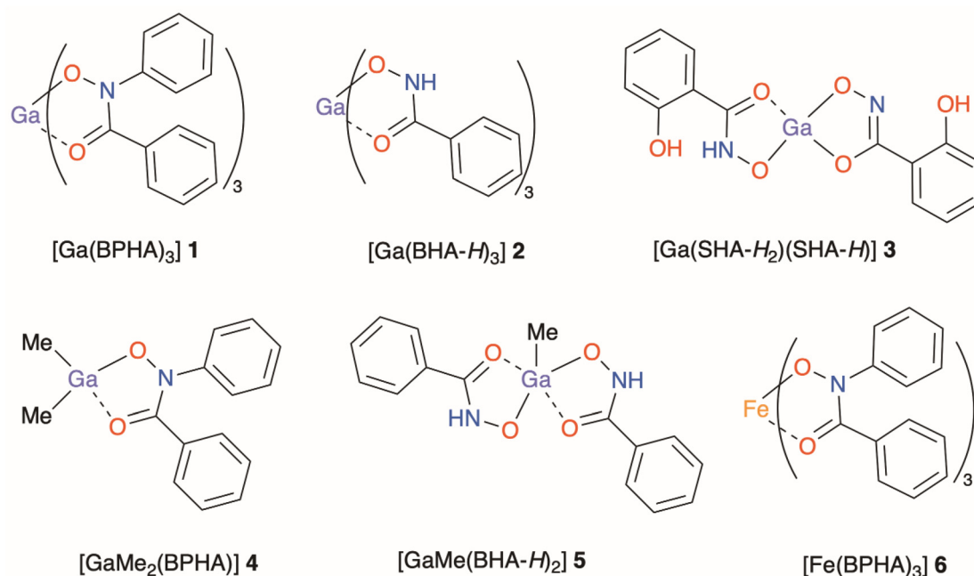
Fig. 2 Complexes synthesised in this study: [Ga(BPHA)_3] 1 , [Ga(BHA-H)_3] 2 , and [Ga(SHA-H_2)(SHA-H)] 3 , [GaMe_2(BPHA)] 4 , [GaMe(BHA-H)_2] 5 and [Fe(BPHA)_3] 6 .
