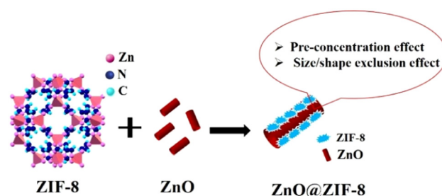
Scheme 4 Schematic representation of the coating of ZnO nanorods using ZIF-8 to yield the ZnO@ZIF-8 composite. Pre-concentration and size/shape exclusion effects are two mechanisms that govern the \text{H}_2 interaction/permeability in the ZnO@ZIF-8 composite based \text{H}_2 chemiresistor.
