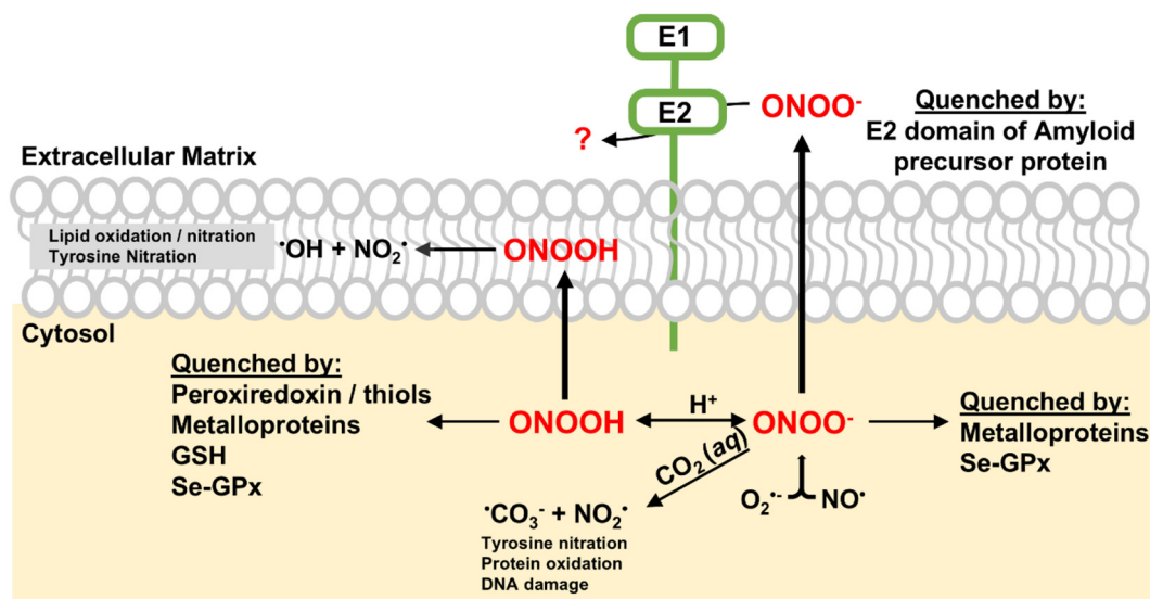
Scheme 1 Possible pathways and targets of ONOO - . ONOO - reacts rapidly with CO 2 , leading to the formation of NO 2 and CO 3 - radicals. NO 2 can react with biomolecules, resulting in nitrated compounds. Alternatively, ONOOH can undergo slow homolysis to generate • OH and NO 2 radicals, causing lipid oxidation and tyrosine nitration. ONOO - can be quenched by various proteins such as peroxiredoxin (Prx), heme-containing proteins and selenium-containing protein glutathione peroxidase (Se-GPx), mitigating its cellular damage.
