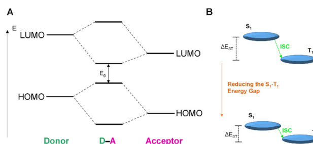
Fig. 5 (A) Schematic diagram presenting the HOMO–LUMO energy levels of donor–acceptor molecules and the molecular interaction between them. (B) A physical model representing the S_1 – T_1 ISC method and the proposed tactic in donor–acceptor molecules. Adapted from ref. 69.
