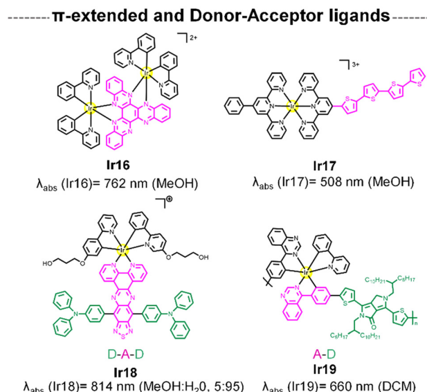
Fig. 4 Structure of Ir complexes with of \pi -extended and donor–acceptor-type N ^ N ligand and its absorption wavelengths.
