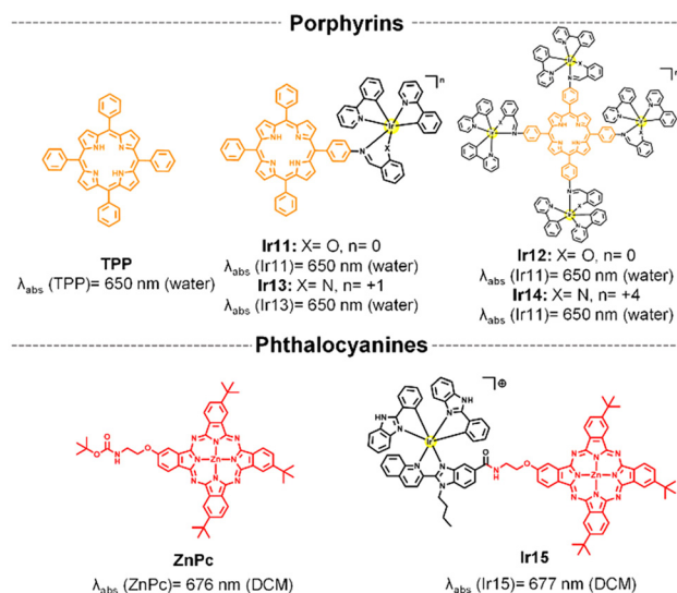
Fig. 3 Structure of porphyrinoid compounds and their Ir-based conjugates.
