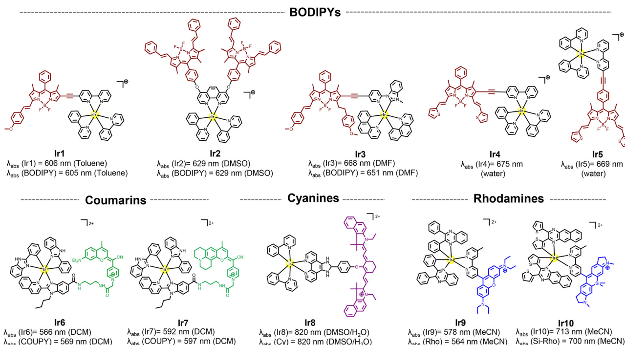
Fig. 2 Selected structures of Ir(III) complexes functionalized to different organic fluorophores and their reported absorption wavelengths.
