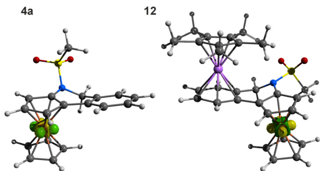
Fig. 6 Electron density changes associated with electron removal, \rho(\text{M}^+) - \rho(\text{M}) , mapped at the geometry of the parent species M ( \text{M} = \mathbf{4a} and the cation of 12 ); isosurfaces at \pm 0.02 a.u. are shown. For details, see the ESI.†
