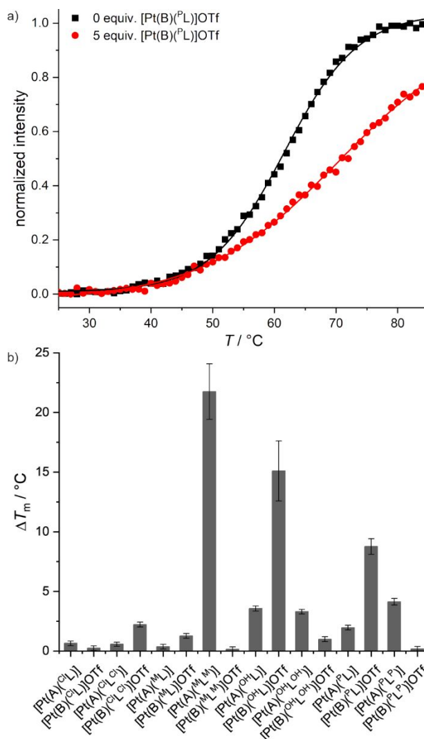
Figure 6 a) Melting curves of FAM- bcl2 -mid-DABCYL in the absence (black) and presence (red) of 5 equiv. of [Pt(B)( P L)]OTf; b) melting point increase ( \Delta T_m ) of FAM- bcl2 -mid-DABCYL upon the addition of 5 equiv. of the respective metal complexes. Conditions: DNA (0.2 \mu M), LiCl (95 mM), KCl (5 mM), MOPS (5 mM, pH 7.4), \lambda_{exc} = 490 nm, \lambda_{em} = 520 nm.
