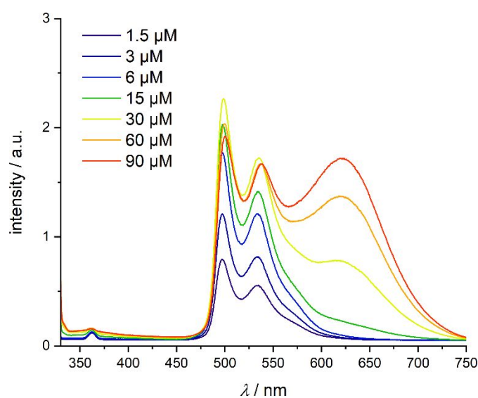
Figure 3 Concentration-dependent emission spectra of [Pt(A)( M L)]. Conditions: metal complex (1.5 – 90 \mu M), 20 °C, \lambda_{\text{exc}} = 340 nm.
