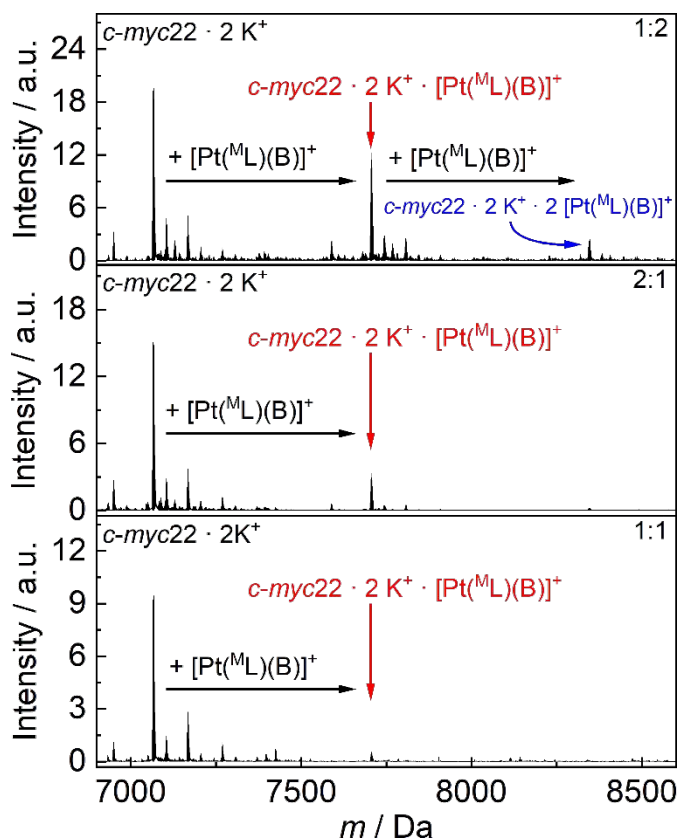
Figure 7 Deconvoluted cryo-ESI-MS spectra of c-myc22 and [Pt(B)(M)L]OTf in DNA:complex ratios of 1:1 (bottom), 2:1 (middle) and 1:2 (top).
