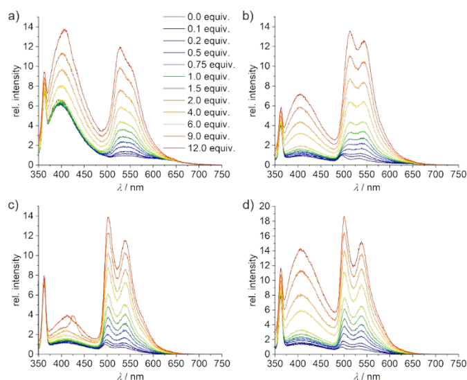
Figure 4 Emission spectra of a) [\text{Pt}(\text{A})^{(\text{Cl})\text{Cl}}] and b) [\text{Pt}(\text{A})^{(\text{Cl})\text{L}}] upon stepwise addition of c-myc22 (0–12 equiv.). Emission spectrum of [\text{Pt}(\text{B})^{(\text{OH})\text{L}}]\text{OTf} upon stepwise addition of c) c-kit and d) H-Telo (0–12 equiv.). Conditions: metal complex (1 \mu\text{M} ), LiCl (90 mM), KCl (10 mM), MOPS (5 mM, pH 7.4), 20 ^{\circ}\text{C} , \lambda_{\text{exc}} = 340 \text{ nm} .
