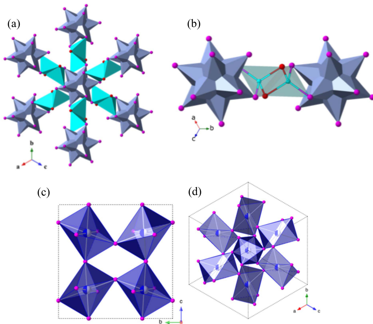
Fig. 3 The (a) polyhedral view of [B_{12}Se_6]^{2-} icosahedron cluster extended along [111] direction, (b) bridging of SiSe_4 tetrahedra between two [B_{12}Se_6]^{2-} clusters, and (c and d) a representation of NaSe_6 octahedra and their connectivity with its neighboring NaSe_6 units.
