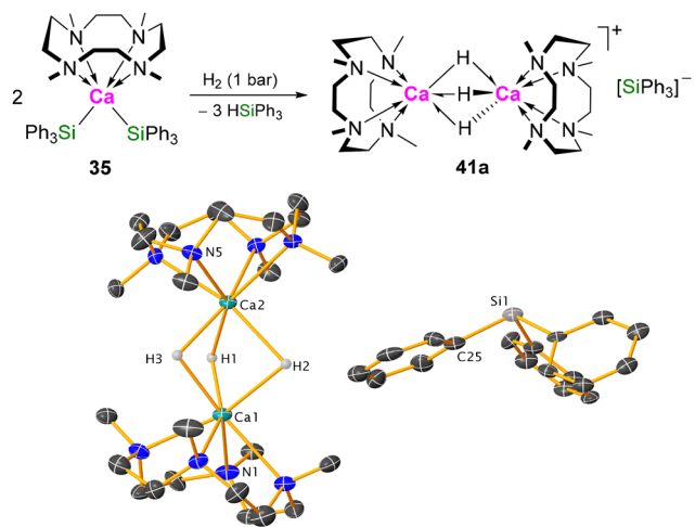
Scheme 10 Hydrogenolysis of compound 35 and molecular structure of dicationic calcium trihydride silyl complex 41a .
