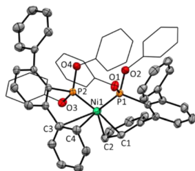
Scheme 2 (A) Synthesis of \text{NiP}_2 complexes 3 and 4 . (B) Improved synthetic route for [\text{Ni}(\text{PMe}_2\text{Ar}^{\text{DtbpP}2})_2] , 2 . (C) Molecular structure of 4 . Hydrogen atoms are omitted for the sake of clarity. Thermal ellipsoids are shown at a 50% probability. Selected bond lengths [Å] and angles [°]: Ni–P1 2.1253(5), Ni–P2 2.1074(5), Ni–C1 2.086(2), Ni–C2 2.211(2), Ni–C3 2.614(2), Ni–C4 2.4261(2), P1–Ni–P2 115.37(2).
