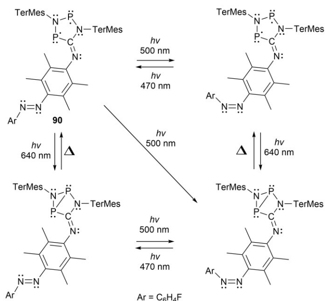
Scheme 17. Novel molecular double switch undergoing constitutional and stereo-isomerization upon irradiation with visible light
