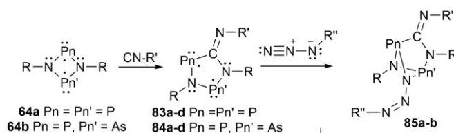
Scheme 9. Reactivity of biradicals of the type [E( \mu NterMes)E'] 2 to generate cyclopentane-1,3-diyl derivatives ( 83a-d , 84a-d ), and Staudinger-type adducts ( 85a-b )
