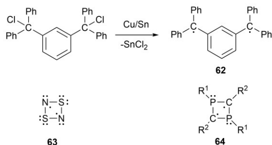
Scheme 2. Pioneering research for main group biradicals
