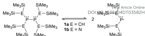
Scheme 1. Equilibrium of the diphosphine and its respective phosphinyl radical in solution
