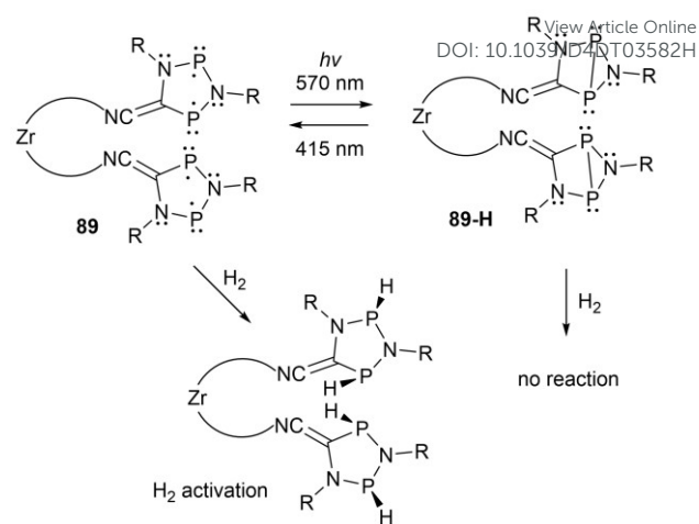
Scheme 16. Photo-switching and H_2 activation investigation of tetraradical 89 and its bis(housane) 89-H
