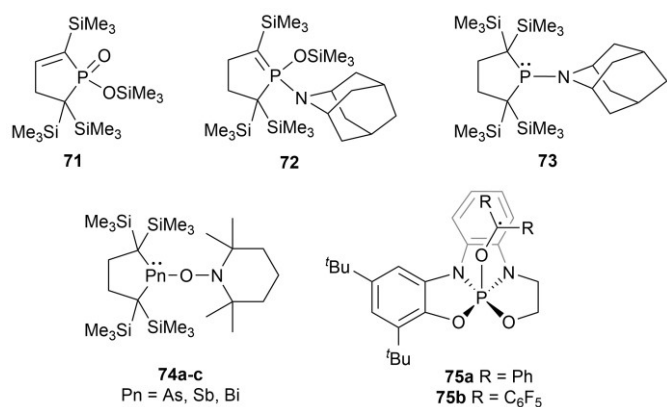
Figure 8. Radical cross-coupling products for Group 15 radicals
