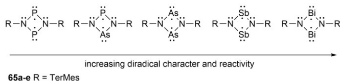
Scheme 3. Altering properties in four-membered biradical ring systems by changing the pnicogen atom(s).
