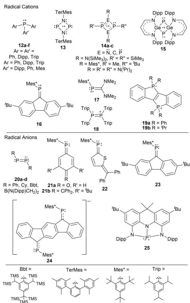
Figure 2. Phosphorus radical cations and radical anions
