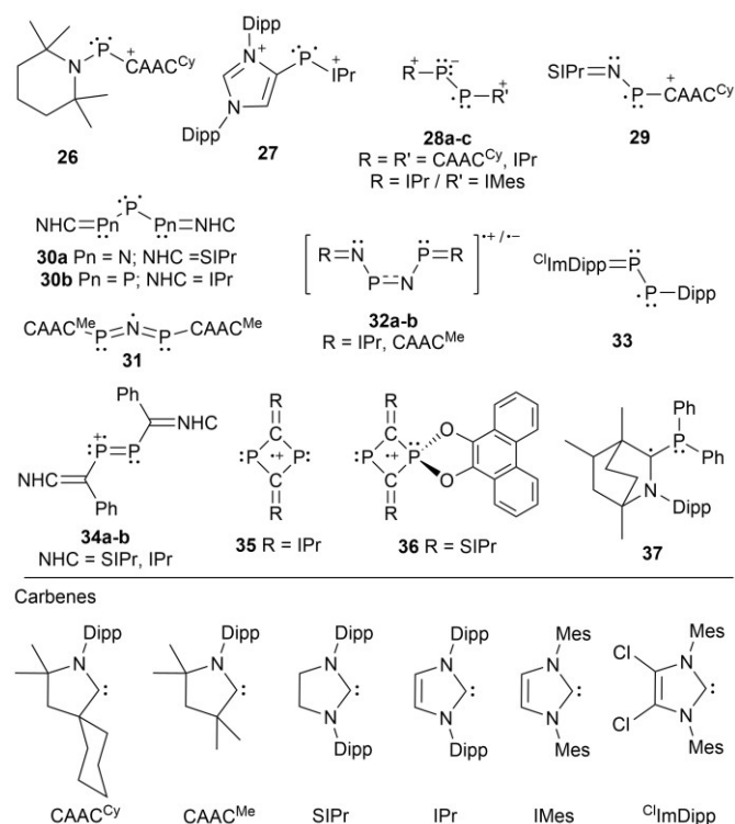
Figure 3. Carbene stabilized phosphorus and phosphorus-nitrogen based radicals
