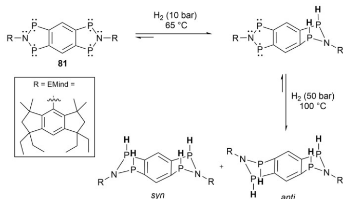
Scheme 7. H 2 activation by the tetradical ( 81 )
