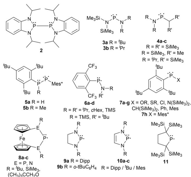
Figure 1. A diphosphine ( 2 ) and phosphinyl radicals ( 3-11 )
