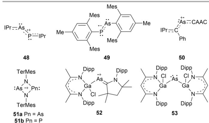
Figure 5. Arsenic-centered radicals generated with new frameworks
