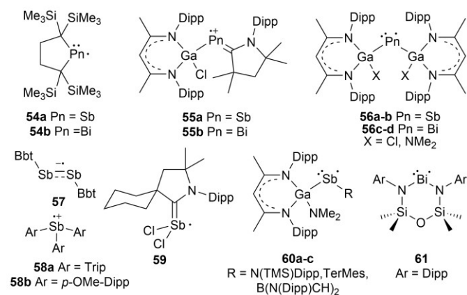
Figure 6. Antimony and bismuth-centered radicals described in the literature
