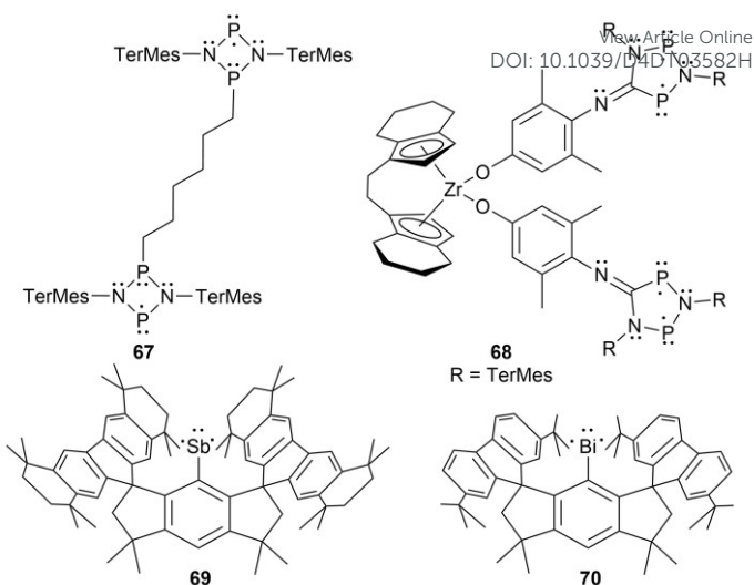
Figure 7. Recent developments of multi-radical centered pnicogens
