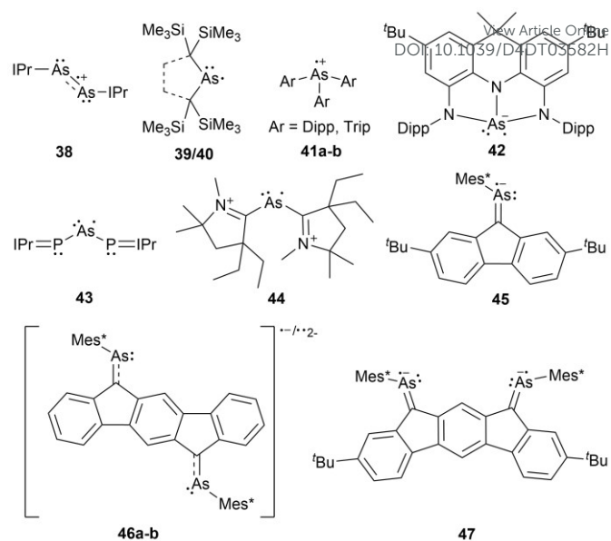
Figure 4. Arsenic-centered radical analogues of phosphorus-based systems
