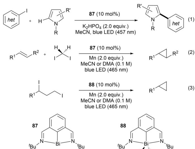
Scheme 15. Light-induced catalytic reactions using bismuth-based catalysts
