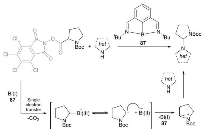
Scheme 14. Bi(I)-Catalyzed formal C(sp^3) -N cross-coupling by radical activation of \alpha -amino redox-active esters
