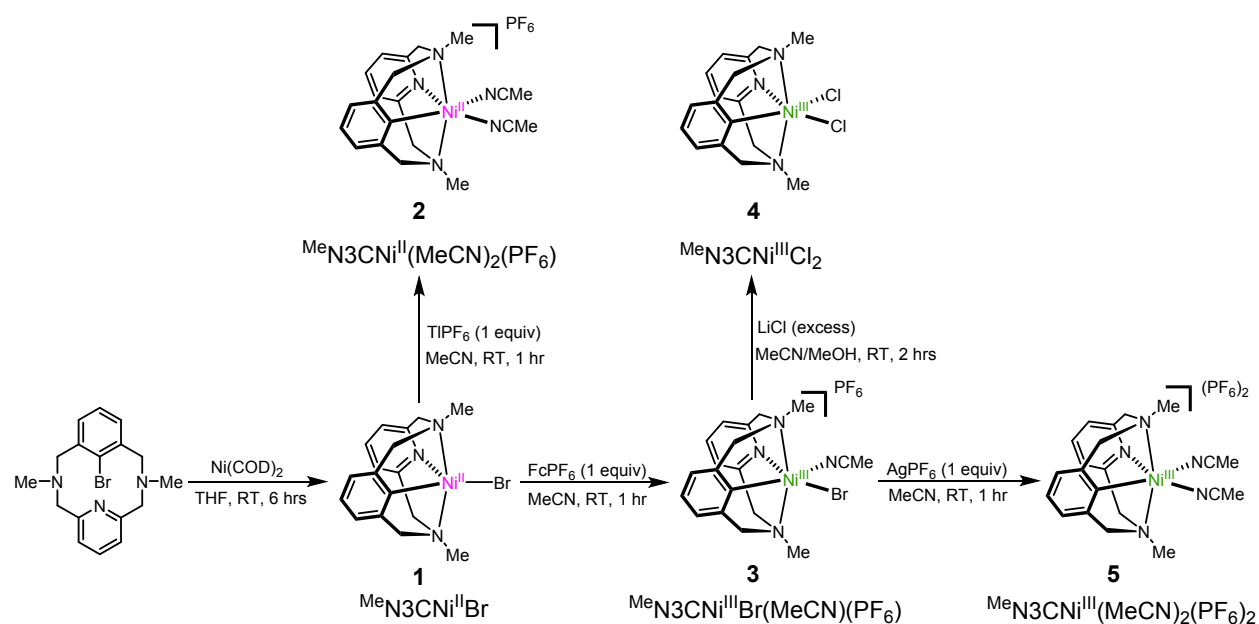
Scheme 1. Synthesis of (Me 3 N 3 C)Ni complexes.
