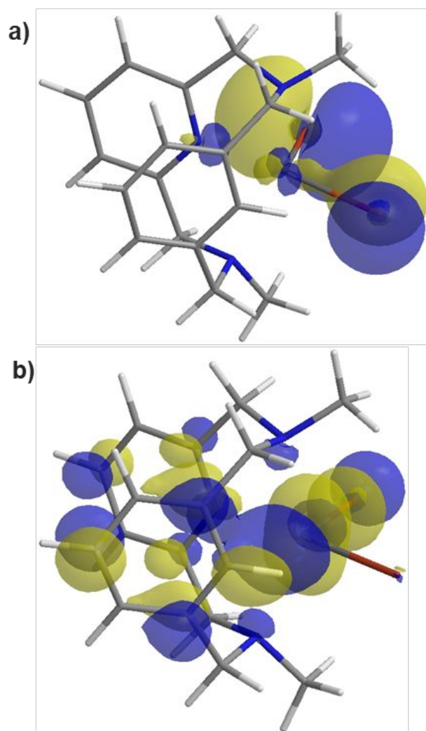
Figure 3. Frontier beta molecular orbitals of 6b a) HOMO and b) LUMO, shown as 0.03 isodensity surfaces, obtained by DFT (B3LYP/def2-TZVPP); the LUMO shows the interaction of C–H bonds with the Ni d orbital.
