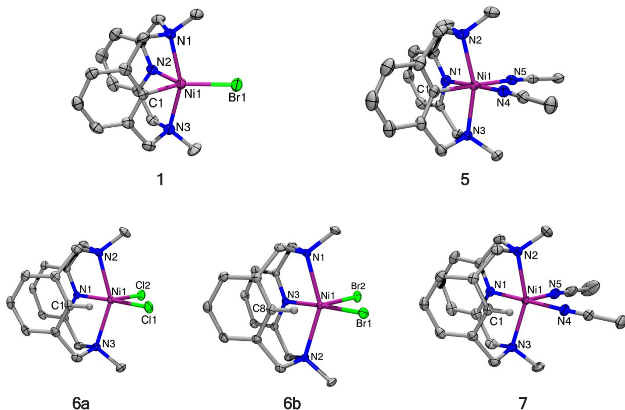
Figure 1. ORTEPs (50% probability thermal ellipsoids) of complexes 1 , dication of 5 , 6a , 6b , and dication of 7 . For clarity, hydrogen atoms and counterions have been omitted. Selected bond distances (Å), 1 : Ni1–N1, 2.291(8); Ni1–N2, 1.981(7); Ni1–N3, 2.276(8); Ni1–C1, 1.954(9); Ni1–Br1, 2.372(2). 5 : Ni1–N1, 1.935(2); Ni1–N2, 2.152(2); Ni1–N3, 2.142(2); Ni1–N4, 1.983(2); Ni1–N5, 1.990(2); Ni1–C1, 1.921(2). 6a : Ni1–N1, 1.993(2); Ni1–N2, 2.233(2); Ni1–N3, 2.242(2); Ni1–C1, 2.539(2); Ni–Cl1, 2.312(5); Ni–Cl2, 2.329(6). 6b : Ni1–N1, 2.223(1); Ni1–N2, 2.255(1); Ni1–N3, 1.985(1); Ni1–C8, 2.482(2); Ni1–Br1, 2.455(4); Ni1–Br2, 2.478(4). 7 : Ni1–N1, 1.971(2); Ni1–N2, 2.179(2); Ni1–N3, 2.169(2); Ni1–N4, 2.023(2); Ni1–N5, 2.037(2); Ni1–C1, 2.412(2).
