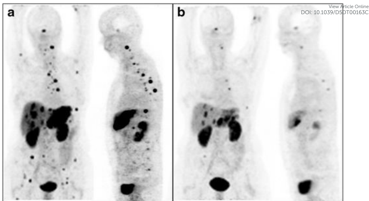
Figure 5: a) [ ^{68}\text{Ga} ]Ga-DOTATOC-PET image of a patient with a tumour in the liver and metastases in the bone marrow as shown in coronal and sagittal maximum intensity projections. B) Reduced tumour burden in the liver after treatment with 10.5 GBq [ ^{213}\text{Bi} ]Bi-DOTATOC, as well as reduction of the bone metastases 6 month after treatment. (Reprinted with permission from [ ^{198} ] Copyright 2014 Springer).
