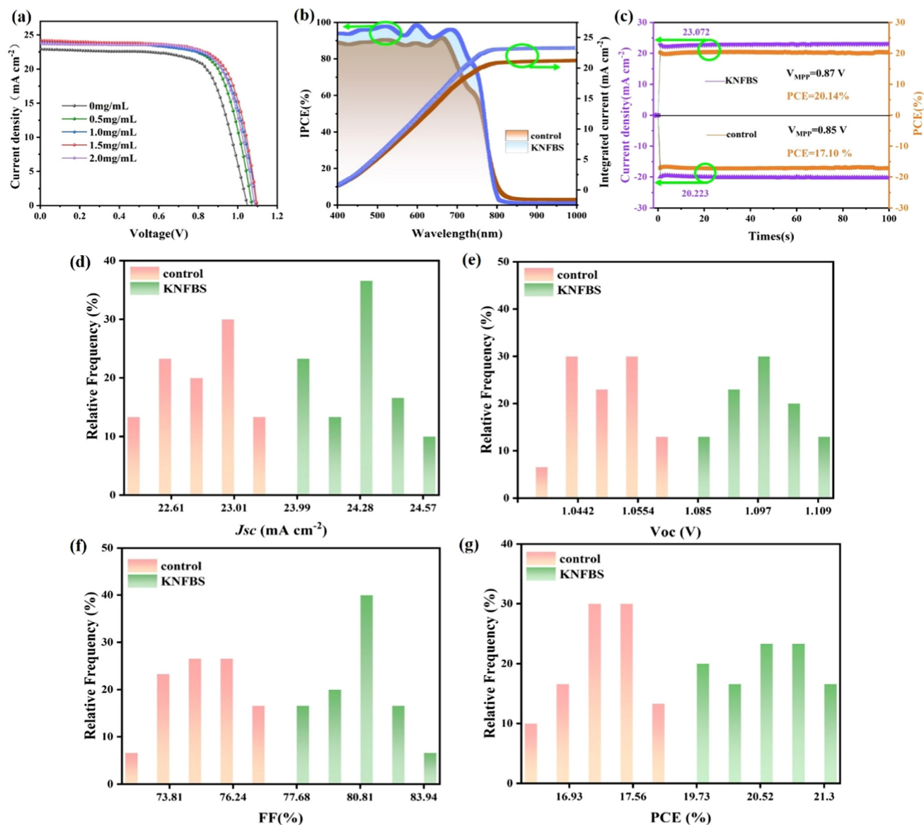
Fig. 2 Photovoltaic performance of pristine and KNFBS-treated devices: (a) J - V curves; (b) IPCE curves. (c) Stabilized PCE and J_{sc} at the maximum power point (MPP) output. Statistical photovoltaic parameter distribution obtained from 30 devices: (d) J_{sc} ; (e) V_{oc} ; (f) FF; (g) PCE.
