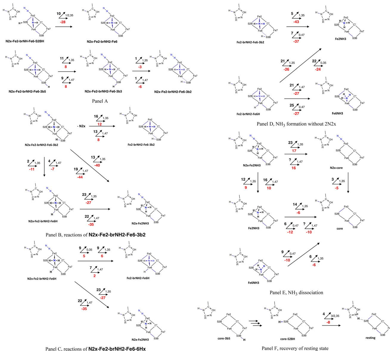
Scheme 3 Calculated reaction potential energies (red) and reaction barriers (black), in kcal mol -1 . Electronic states are marked, as S,35 or S,47. Panel A describes the preparatory steps forming \text{N2x-Fe2-brNH2-Fe6-3b2} from \text{N2x-Fe2-brNH2-Fe6-S2BH} . Panel B describes the three reactions of \text{N2x-Fe2-brNH2-Fe6-3b2} and panel C describes the two reactions of \text{N2x-Fe2-brNH2-Fe6-6Hx} . Panel D contains the steps that form \text{NH}_3 after prior dissociation of \text{N2x} . Panel E describes the \text{NH}_3 dissociation steps from intermediates with and without \text{N2x} , and also the two \text{N2x} dissociation steps with and without bound \text{NH}_3 . Panel F shows recovery of the resting state.
