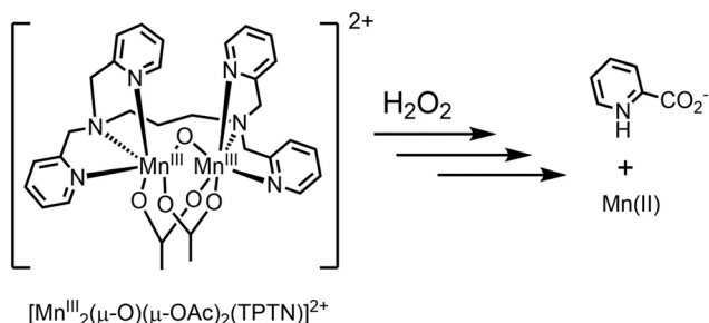
Fig. 9 Decomposition of [Mn_2(\mu-O)(\mu-OAc)_2TPTN]^{2+} to pyridine-2-carboxylic acid.
