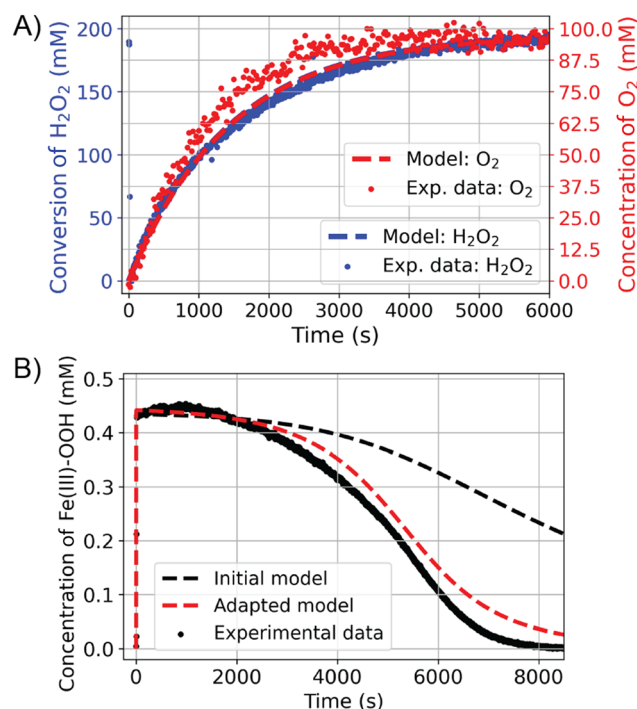
Fig. 7 Reaction progress for the conversion of 400 equiv. of H_2O_2 (0.46 mM [(N_4Py)Fe^{II}(CH_3CN)](OTf)_2 and 190 mM H_2O_2 in methanol). (A) ^3O_2 (red) and H_2O_2 (blue) reaction progress determined by Raman spectroscopy. (B) Concentration of (N_4Py)Fe^{III}-OOH over time from visible absorption spectroscopy. Experimental data are denoted with dots and the modelled data with dashed lines. 17
