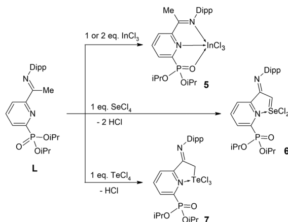
Scheme 5 Synthesis of neutral complex [\text{InCl}_3(\text{L})] ( 5 ) and C–H activation products 2\text{-(C(CH=SeCl}_2\text{)=N(Dipp))}\text{-6-((iPrO)}_2\text{P=O)C}_5\text{H}_3\text{N} ( 6 ) and 2\text{-(C(CH}_2\text{TeCl}_3\text{)=N(Dipp))}\text{-6-((iPrO)}_2\text{P=O)C}_5\text{H}_3\text{N} ( 7 ).
