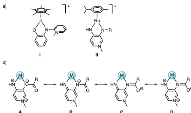
Figure 1. a) Underligated Ir III and Ru II complexes containing pyridinium amidate (PYA) ligands; b) schematic representation of the limiting resonance structures in N,N'-bidentate PYA complexes.
